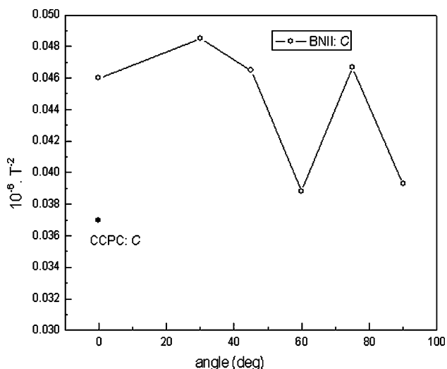
Fig. 5 The measurement direction dependence of the parameter C of BNII and CII
