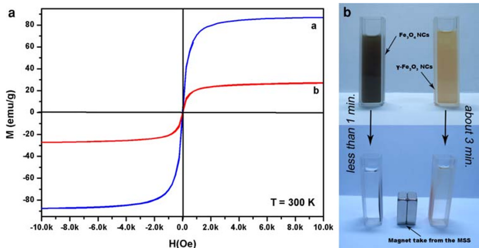
Fig. 6 Hysteresis loops (A) of Fe 3 O 4 nanocages (a) and \gamma -Fe 2 O 3 Nanocages (b); Photographs (B) of the Fe 3 O 4 nanocages and \gamma -Fe 2 O 3 nanocages (dispersed in ethanol solution) before and after magnetic separation by an external magnetic field (this magnet takes from the MSS)
