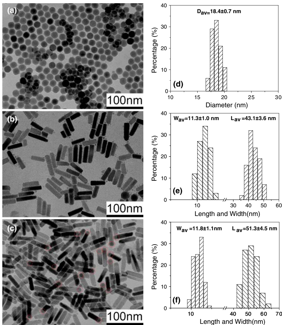
Fig. 2 TEM images of a Cu 2 S nanocrystals, b In 2 S 3 nanorods, and c matchstick-like Cu 2 S–In 2 S 3 heterostructure nanocrystals (part of the heads are marked by the red circle). The panels (d) , (e) , and (f) correspond to the size distribution histograms of the samples used in our work
