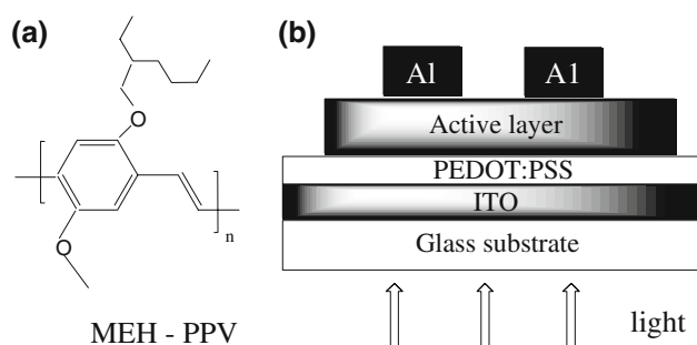
Fig. 1 a Chemical structure of MEH-PPV; b Schematic illustration of the hybrid photovoltaic device structure
