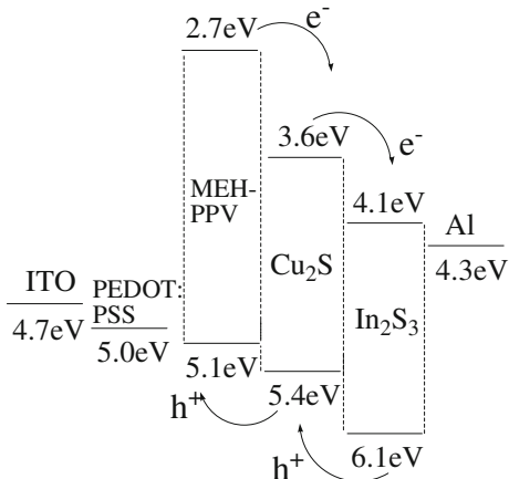
Fig. 6 Energy level diagram showing the charge transfer for the MEH-PPV:Cu 2 S–In 2 S 3 hybrid photovoltaic device
