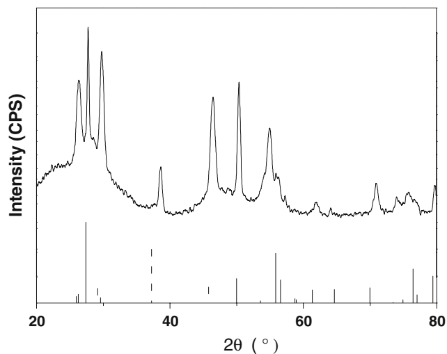
Fig. 3 XRD pattern of the matchstick-like heterostructure nanocrystals. The solid and dash lines shown in below the frame correspond to the standard \text{In}_2\text{S}_3 (JCPDS: 73-1366) and \text{Cu}_2\text{S} (JCPDS: 84-0206), respectively
