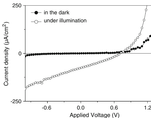
Fig. 4 Current density–voltage characteristics of the MEH-PPV: \text{Cu}_2\text{S} – \text{In}_2\text{S}_3 hybrid device in the dark (closed circles) and under illumination (open circles)
