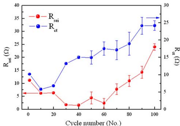
Fig. 4 The resistive components of SEI and charge transfer reaction according to the cycle number, as calculated from previous Nyquist plots by curve fitting
