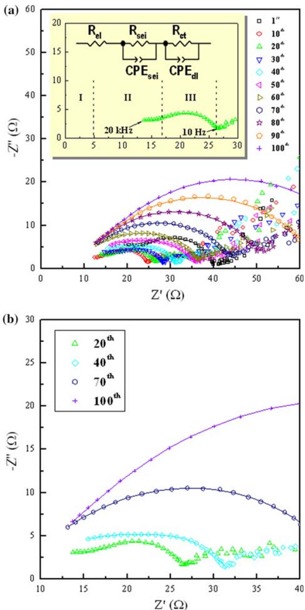
Fig. 3 a Family of Nyquist plots collected from the 1st and 10th–100th discharged states (at 10-cycle intervals) over a frequency range from 20 kHz to 10 Hz, including an equivalent circuit analog for curve fitting. b Magnified view of Nyquist plots for the 20th, 40th, 70th, and 100th discharged states to show the disappearance of the border between SEI and charge transfer contribution
