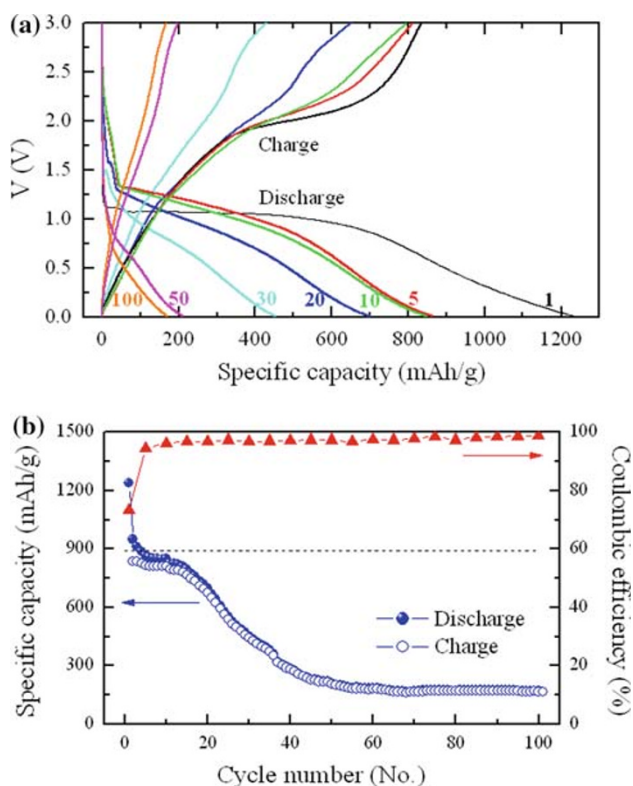
Fig. 2 Galvanostatic electrochemical evaluation of nano-sized \text{Co}_3\text{O}_4/\text{Li} half-cell at a rate of C/5 during 100 cycles: a discharge/charge voltage profiles between 0.01 and 3.0 V at a rate of C/5 , and b plot of discharge/charge capacities against cycle number. The closed and open circular symbols denote the discharge and charge capacities, respectively. The closed triangular symbol indicates coulombic efficiency
