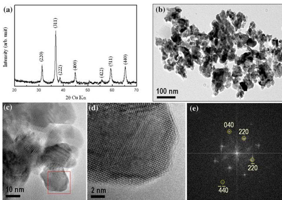
Fig. 1 a XRD pattern of nano-sized \text{Co}_3\text{O}_4 with cubic spinel structure, b and c typical low-magnification images of nano-sized \text{Co}_3\text{O}_4 , d magnified HRTEM images of a selected region in c , and e FFT pattern calculated from a single \text{Co}_3\text{O}_4 nanoparticle
