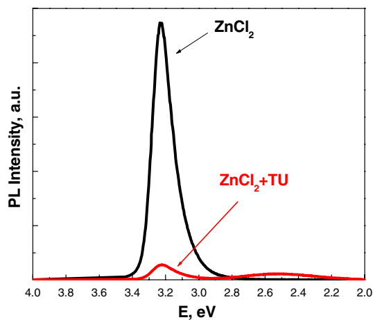
Fig. 8 Room-temperature PL spectra of the ZnO nanorods prepared from solutions of ZnCl 2 and ZnCl 2 containing thiocarbamide at molar ratio of Zn:tu = 1:0.25, [Zn 2+ ] = 0.05 mol/L
