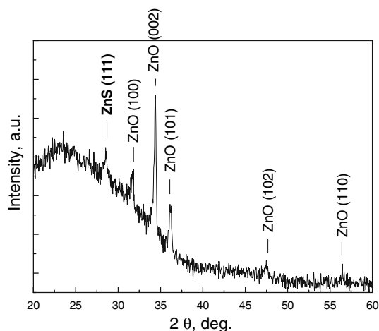
Fig. 5 XRD pattern of the sample obtained from solution containing ZnCl 2 and thiocarbamide (Zn:tu = 1:0.5), [Zn 2+ ] = 0.1 mol. Diffractogram was recorded using parallel beams
