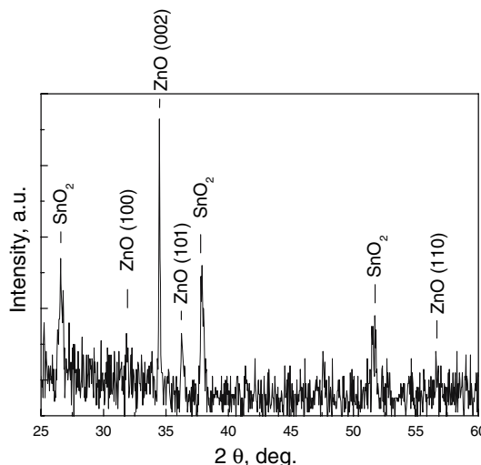
Fig. 3 XRD pattern of the samples deposited from solutions containing ZnCl 2 and thiocarbamide (Zn:tu = 1:0.25), [Zn 2+ ] = 0.1 mol/L
