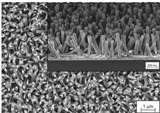
Fig. 2 The SEM surface and cross-sectional views (inset) images of ZnO nanorods obtained from solution with thiourea addition at molar ratio of Zn:tu = 1:0.25, [Zn 2+ ] = 0.1 mol/L
