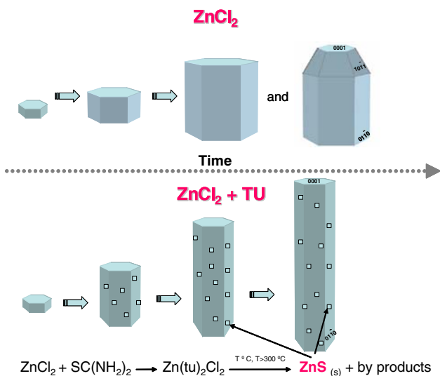
Fig. 7 Schematic illustration of the possible growth mechanism for the formation of ZnO nanorods from the ZnCl 2 solutions without and with thiourea
