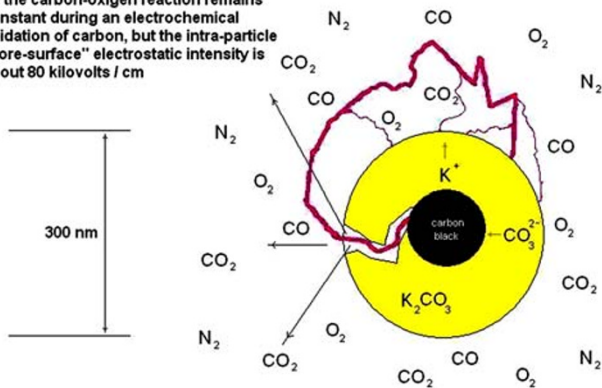
Fig. 2 Nanocapsules, containing a core reducing agent and surface electrolyte layer, form short-circuited aerosol nanobatteries
