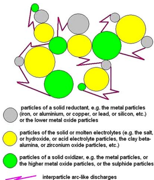
Fig. 1 Mixed sintered nanoaggregates of condensed smoke particles, containing solid reductant, electrolyte and oxidizer, inevitably form short-circuited aerosol nanobatteries
