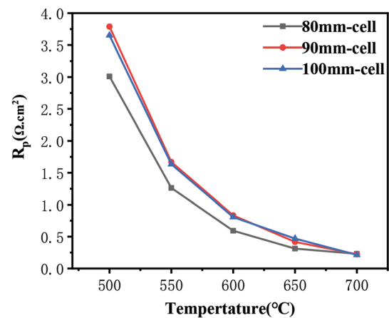
Fig. 11 Polarization resistance as a function of temperature for the three cells
