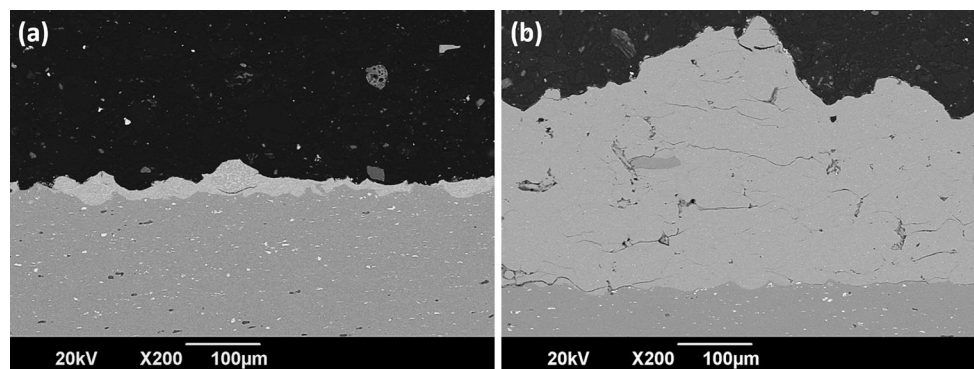
Fig. 11 Cross section BSE images of the coating deposition of as-received particles (a) and solution heat-treated (b) and of AA7075 powder showing a high thickness (300 \mu\text{m} ) in the second case
