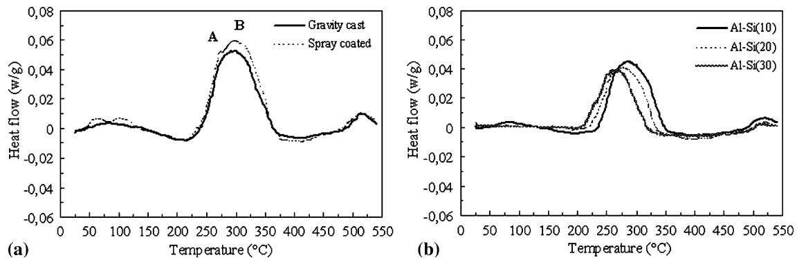
Fig. 4 Results of DSC analysis: (a) Al-Si matrix alloys and (b) Plasma-sprayed Al-Si/SiC composites
