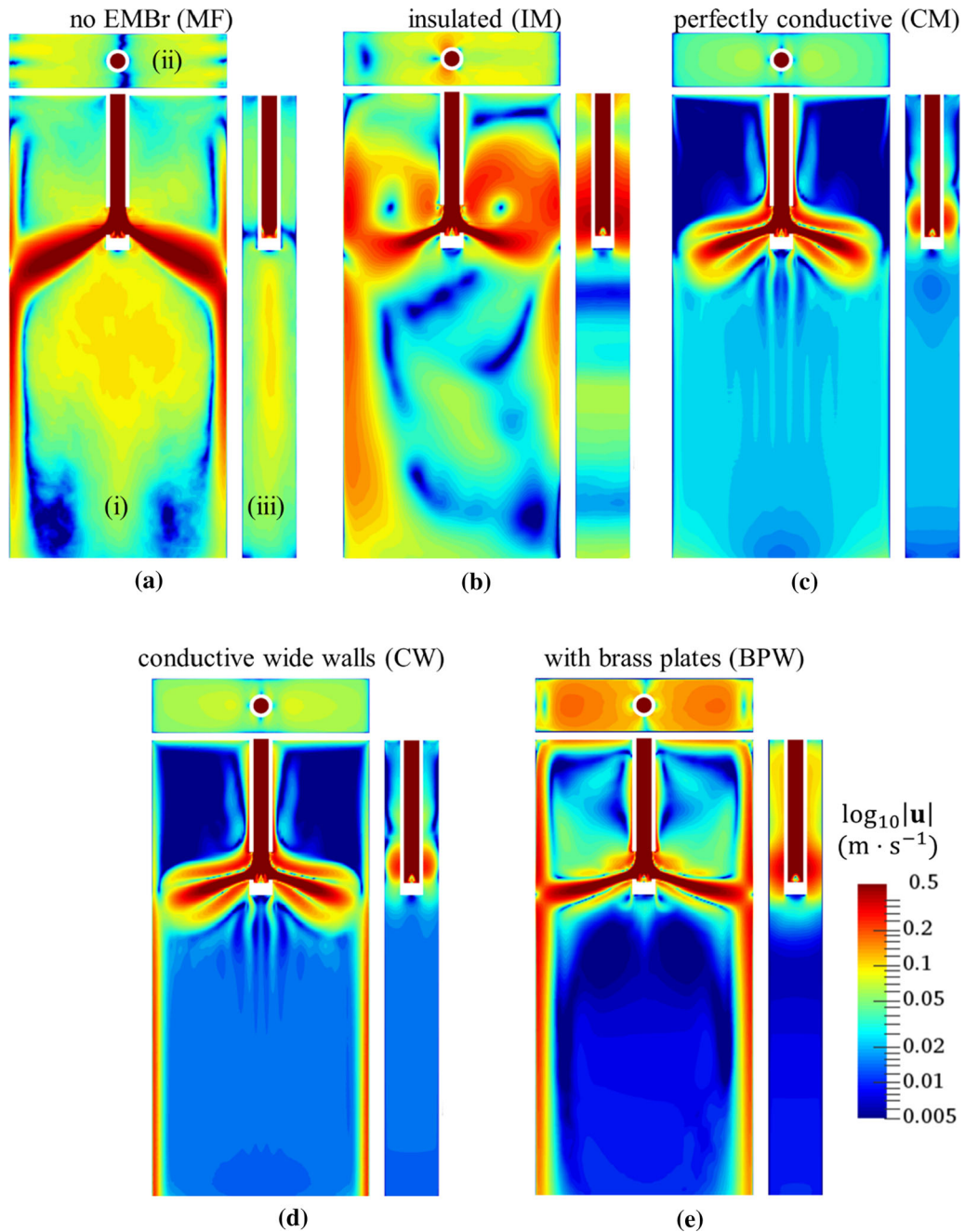
Fig. 7—Time-averaged (39 seconds window) velocity magnitude |\mathbf{u}| : (i) wide side mid-plane, (ii) top surface; (iii) narrow side mid-plane. The results are shown for the following cases: (a) no magnetic field applied; EMBr simulations (b) with all walls insulated; (c) all walls conductive; (d) with conductive wide walls; and (e) with attached brass plates.
