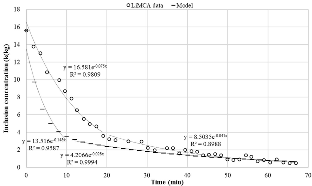
Fig. 13—Settling trend of the inclusions monitored by LiMCA after addition of \text{Al}_2\text{O}_3\text{:MgO} particles.
