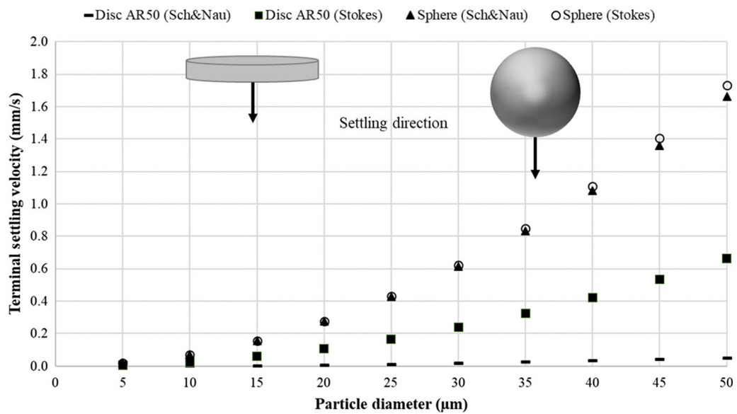
Fig. 2—Calculated velocities of settling discs with Ar = 50 and spheres by using Stokes and Schiller and Naumann [20] drag.
