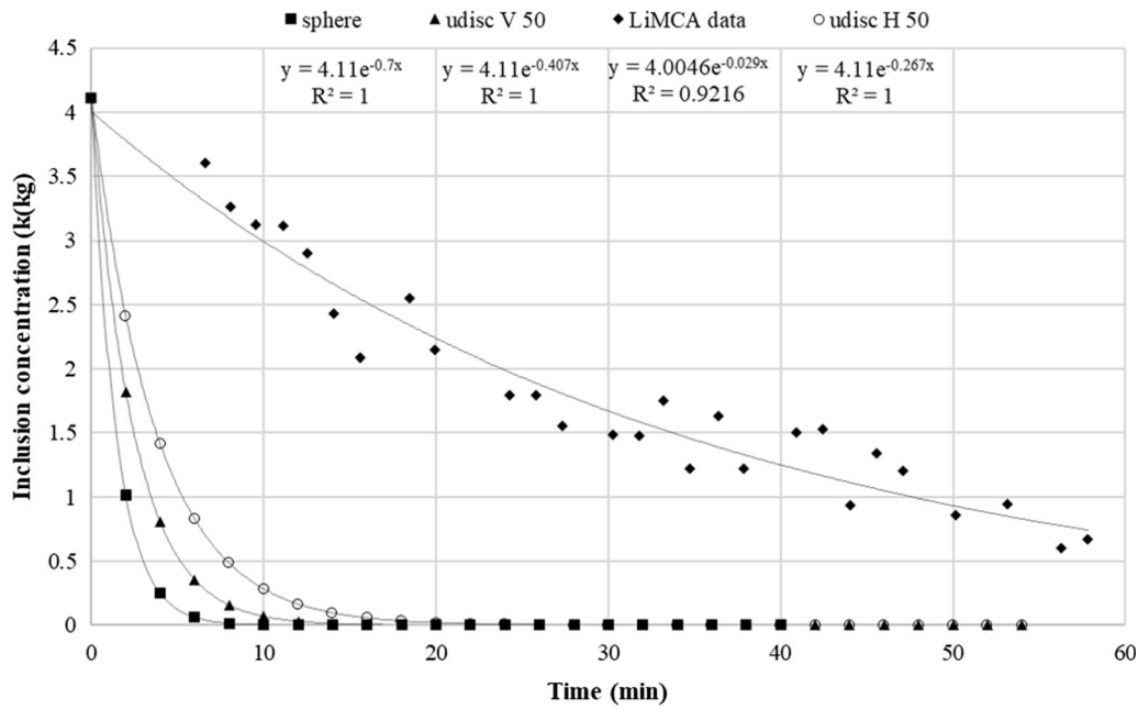
Fig. 9—Free settling behavior of discs and spheres in comparison with the LiMCA data.
