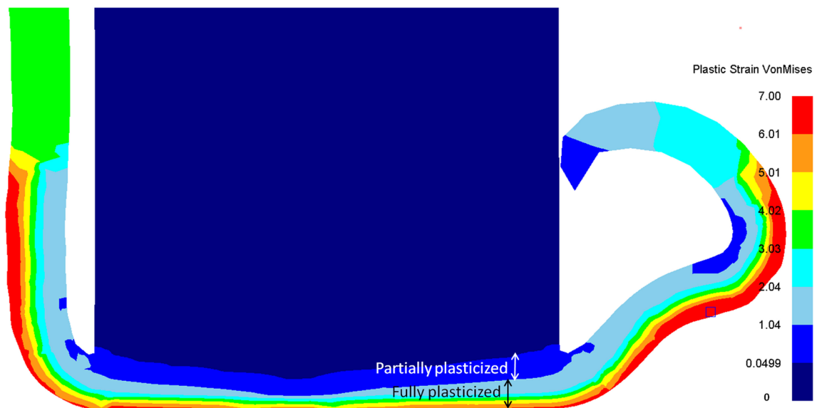
Fig. 8—FE-predicted Von Mises plastic strain field for an IFW weld model.
