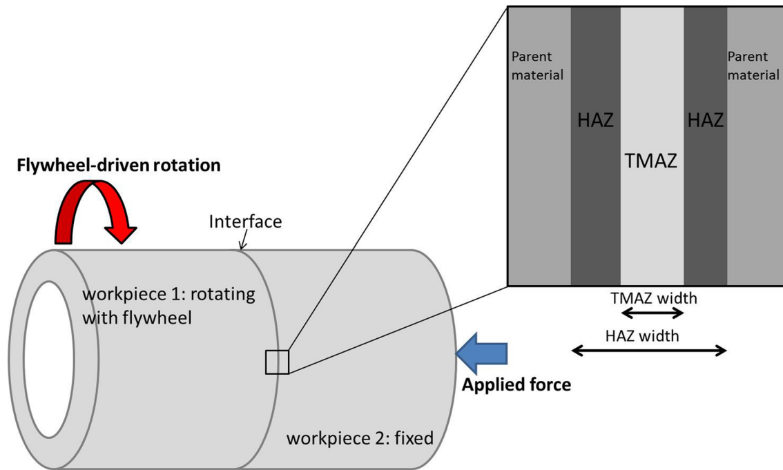
Fig. 1—Schematic of an inertia weld on a hollow cylinder, showing a macroscale representation of the banding of parent, HAZ, and TMAZ materials.
