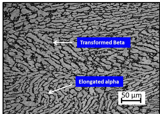
Fig. 2—Elongated \alpha grain in a transformed \beta matrix at \times 50 magnification.
