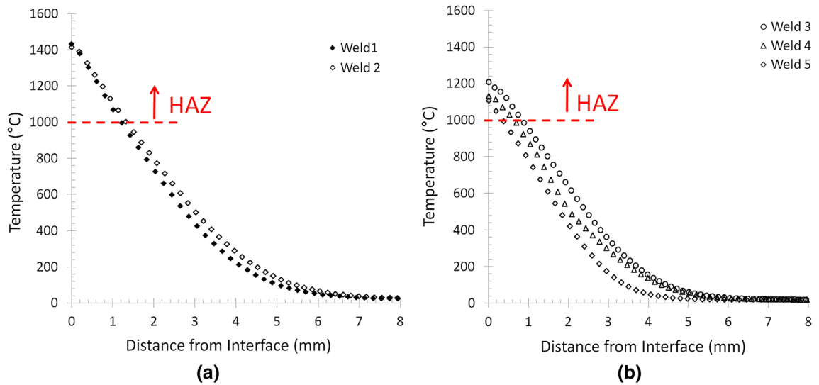
Fig. 7—Predicted thermal profiles for one half of the weld, at steady-state section of welding time, for FE models by varying (a) the applied pressure and (b) the initial rotational speed during the IFW process.
