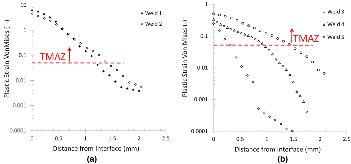
Fig. 9—Predicted Von Mises plastic strain profiles for one half of the weld, at the steady-state section of welding time, for FE models; (a) varying the applied pressure and (b) varying the initial rotational velocity during the IFW process.
