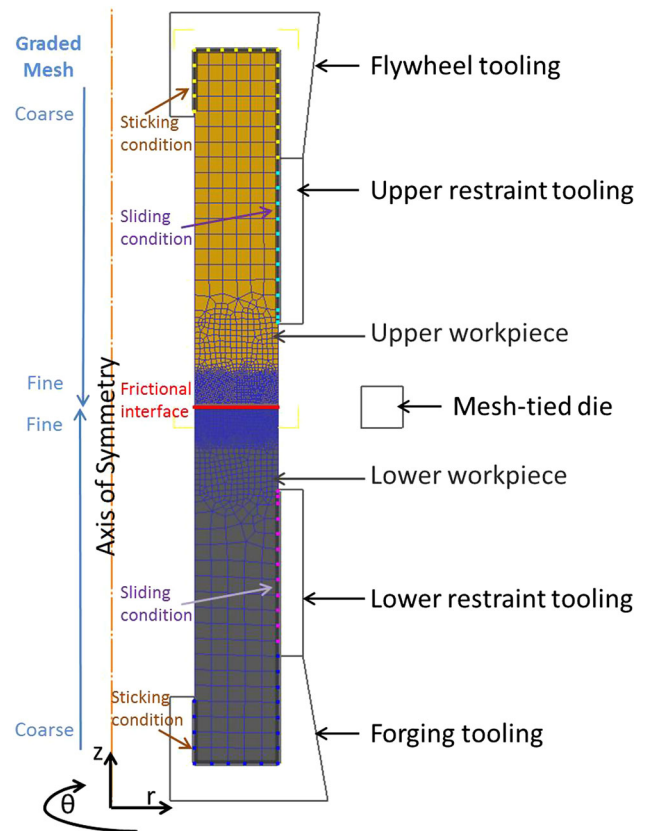
Fig. 3—An example of the FE modeling setup for the IFW modeling in Deform v11.0.
