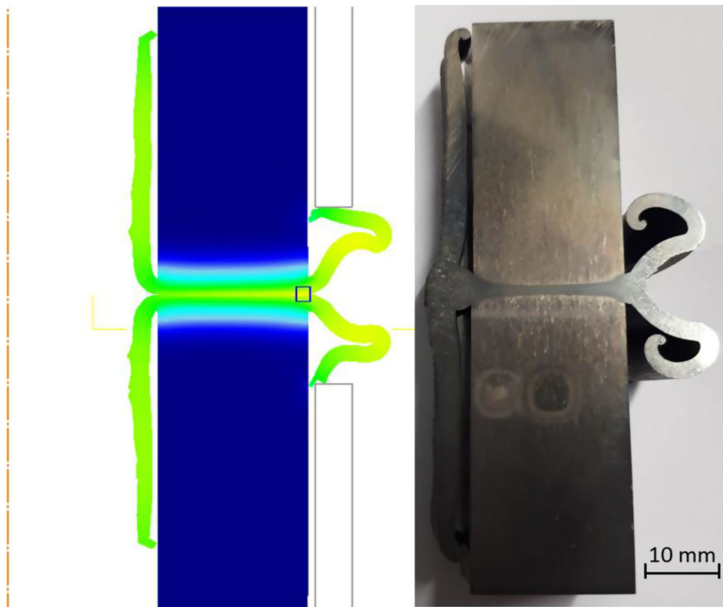
Fig. 5—Comparison of macroscale flash appearances within the model and the real process.
