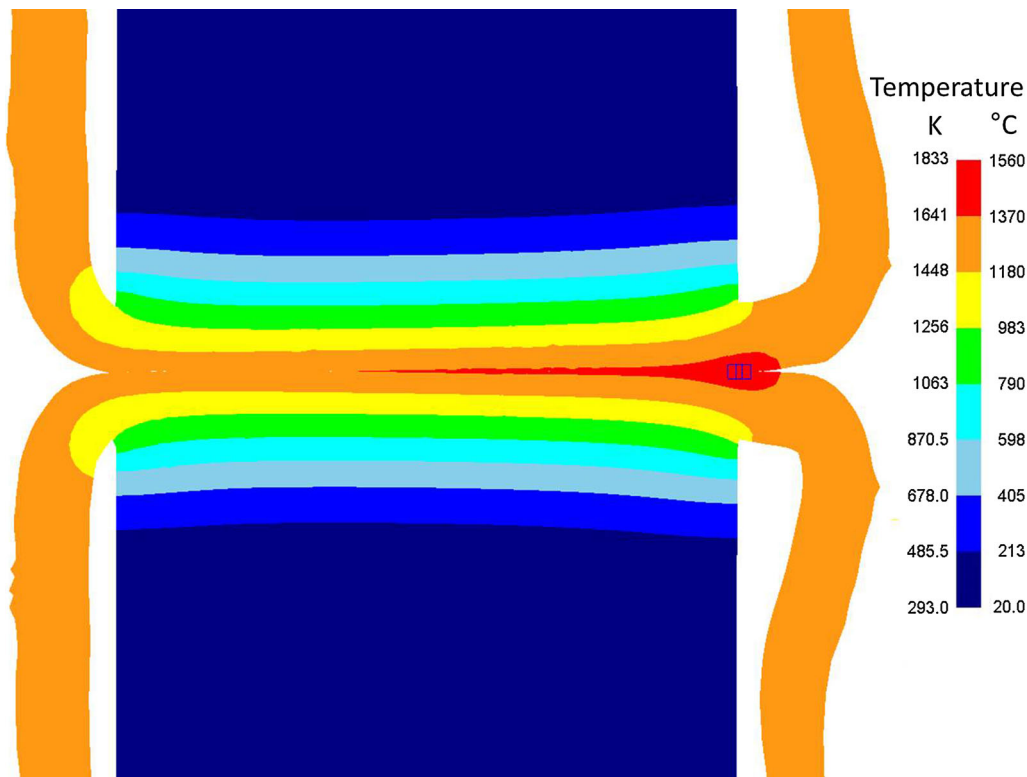
Fig. 6—FE-predicted thermal profile for a weld model. The scale indicates temperatures from RT up to 1833 K (1560 °C). Note that the green-to-yellow boundary indicates the \beta -transus temperature.
