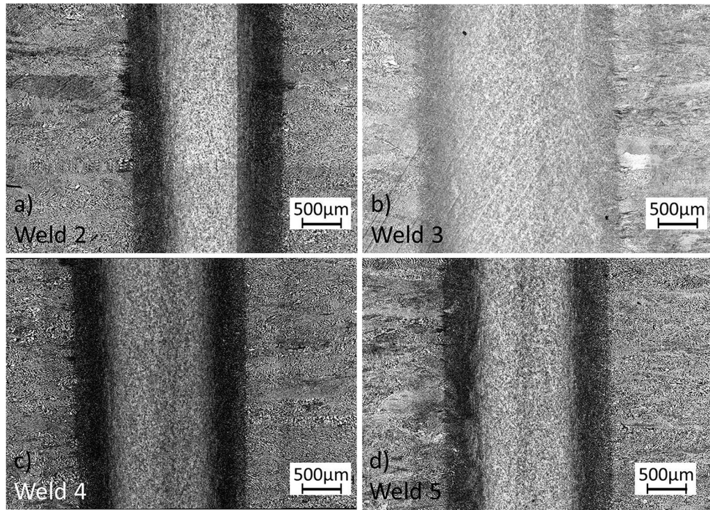
Fig. 4—Optical microscopy illustrating the parent, HAZ and TMAZ zones measured from (a) Weld 2, (b) Weld 3, (c) Weld 4, (d) Weld 5.
