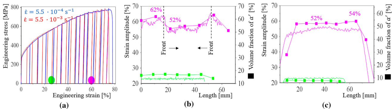
Fig. 5—(a) Stress–strain curves of displacement-controlled, loading–unloading test of 304 at room temperatures, GL = 30 mm (blue: 1 mm/min, \dot{\epsilon} = 5.5 \times 10^{-4} \text{s}^{-1} and red: 10 mm/min, \dot{\epsilon} = 5.5 \times 10^{-3} \text{s}^{-1} ); (b) and (c) volume fraction of martensite \alpha' (squares) vs strain amplitude along the specimen axis measured after unloading cycles (for green and magenta dot, respectively). (b) Stable propagation of the strain-localized band is observed for strain rate \dot{\epsilon} = 5.5 \times 10^{-4} \text{s}^{-1} (arrows); (c) Uniform distribution of strain amplitude and volume fraction of martensite \alpha' is observed for strain rate \dot{\epsilon} = 5.5 \times 10^{-3} \text{s}^{-1} (Color figure online).
