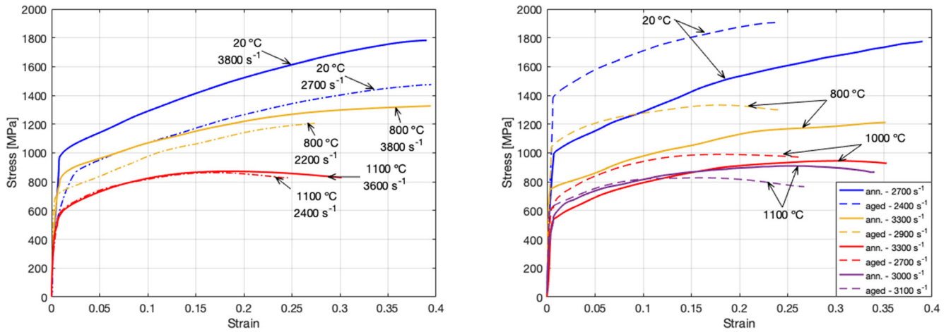
Fig. 6—True stress–strain curves of alloy 718 in annealed state for different strain rates at 20 °C, 800 °C and 1100 °C.
