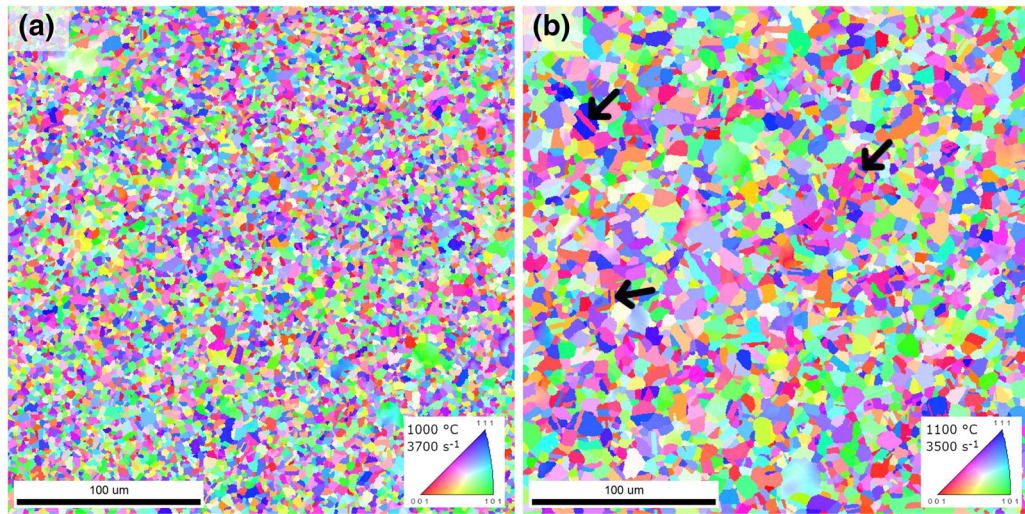
Fig. 17—Inverse Pole Figures (IPF) obtained by EBSD analysis of alloy 718 in aged state (a) deformed at 1000 °C and 3700 s -1 (b) deformed at 1100 °C and 3500 s -1 —black arrows indicate twins (Color figure online).
