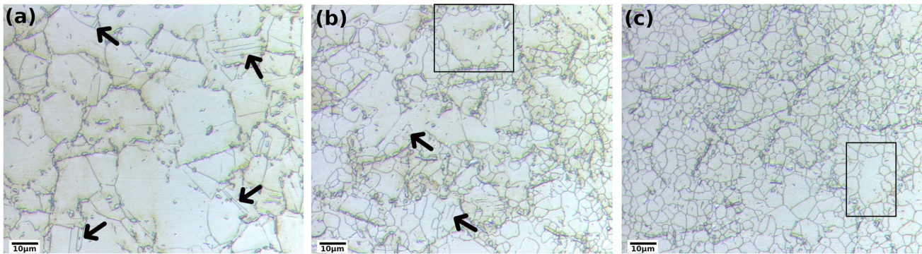
Fig. 15—Optical micrographs of alloy 718 in annealed state deformed at 1000 °C and 3000 s -1 for three different zones in the same sample: (a) non-recrystallized (b) partially recrystallized (c) mostly recrystallized—black arrows indicate twins—black frames show necklace structures.
