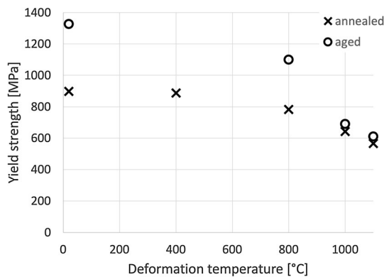
Fig. 18—Yield strength vs temperature for alloy 718 in annealed and aged states.
