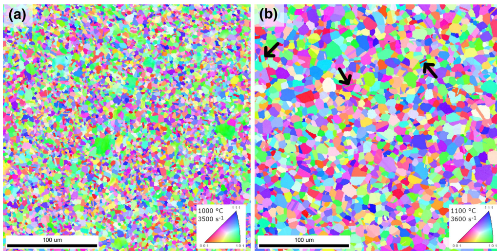
Fig. 16—Inverse Pole Figures (IPF) obtained by EBSD analysis of alloy 718 in annealed state (a) deformed at 1000 °C and 3500 s -1 (b) deformed at 1100 °C and 3600 s -1 —black arrows indicate twins (Color figure online).
