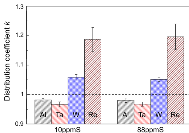
Fig. 16—Results of Scheil-type analysis on 10ppmS and 88ppmS. The average fitted distribution coefficient of eight analyzed axes connecting the dendrite cores to the final solidification point is shown for Al, Ta, W, and Re with error bars indicating standard deviation.
