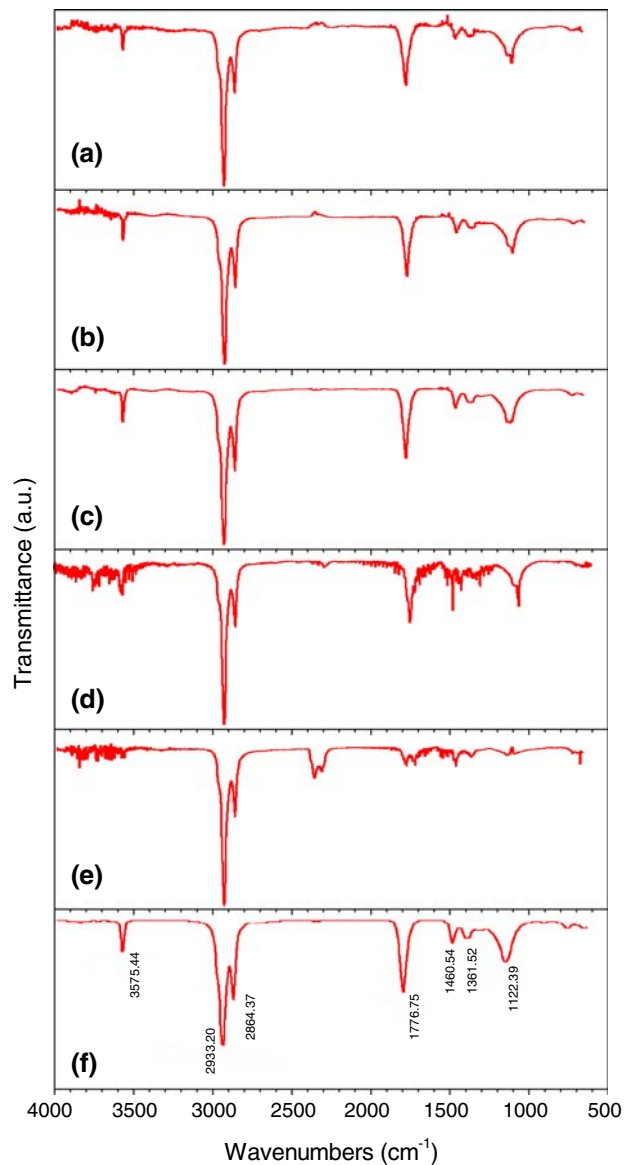
Fig. 6—FTIR spectra of evolved gas from TGA experiments: (a) stearic acid, (b) stearic acid + Al, (c) stearic acid + \text{Al}_2\text{O}_3 , (d) stearic acid + MgO (200 °C to 250 °C), (e) stearic acid + MgO (350 °C to 450 °C), and (f) stearic acid spectrum (Nicolet Vapor Phase Library).
