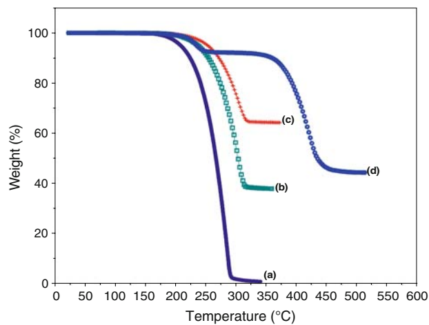
Fig. 5—TGA curves of (a) stearic acid, (b) stearic acid + Al, (c) stearic acid + \text{Al}_2\text{O}_3 , and (d) stearic acid + MgO.
