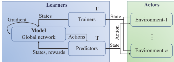
Fig. 6 Basic framework of GA3C
