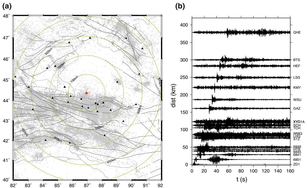
Fig. 5 a Locations of the air-gun source (red star) and permanent seismic stations (black triangles) in Xinjiang, China. Gray circles indicate seismicity from 1970 to 2013. Blue lines are fault traces. Large green circles denote the distance from the source. b Waveform cross section (vertical component) recorded by permanent stations. Waveforms are stacked for 100 air-gun shots. Station names are labeled at the right side of each trace. After Wang et al. (2013)
