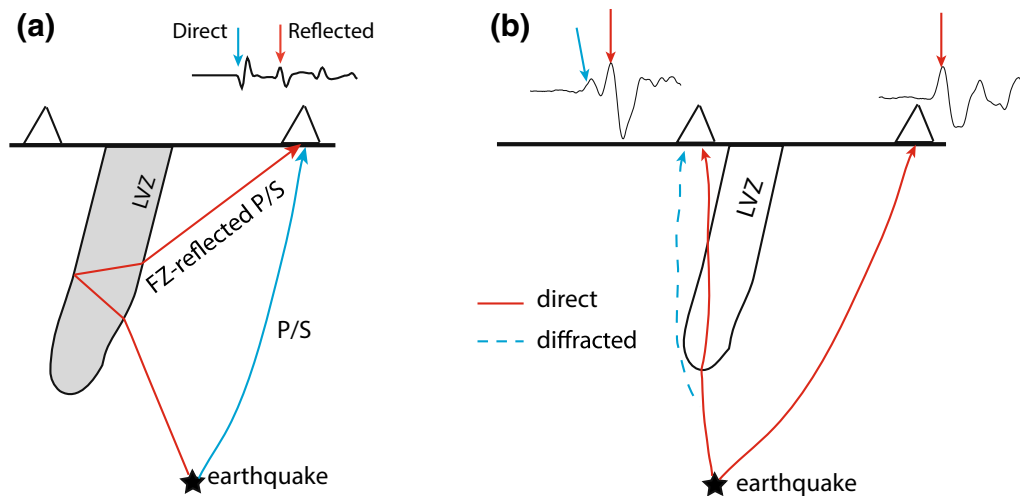
Fig. 2 Schematic plots for the direct and FZ-reflected P and S waves (a) and FZ-diffracted body waves (b). After Yang and Zhu (2010a)
