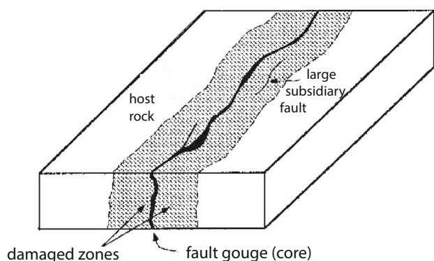
Fig. 1 A schematic plot of a typical fault zone, after Chester and Logan (1986)
