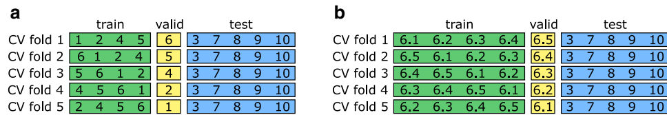
Fig. 1 Overview of the used CV schemes and the distribution of patients among the individual sets. a CV scheme for scenarios one (250 training images) and two (150 training images). Scenario two only uses 60% of
