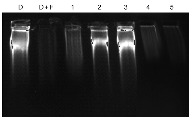
Figure 4 DNA protection assay of extracts from respective endophytic fungus. D. Calf thymus DNA; (D + F). DNA + Fenton's reagent; 1. A. tenuissima ; 2. F. chlamydosporum ; 3. N. hematococca ; 4. B. specifera ; 5. A. terreus .
