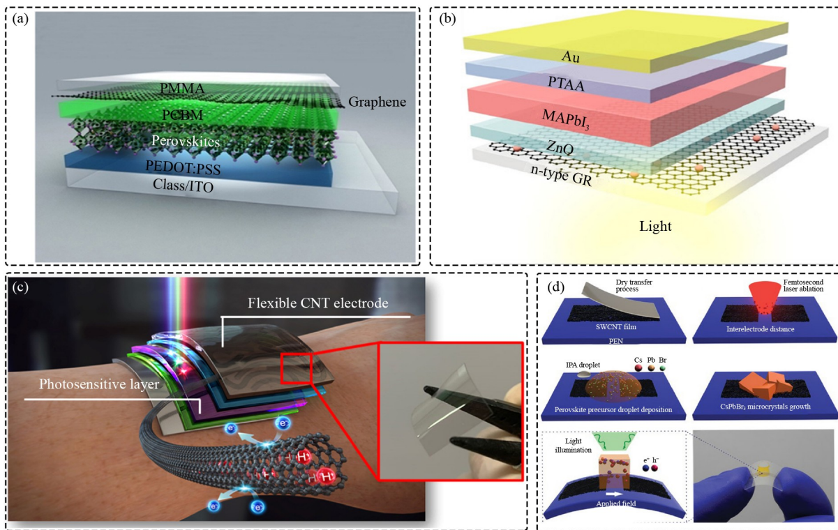
Fig. 11 Fabrication processes and device structures of flexible photodetectors with (a) top grapheme electrode [100], (b) bottom grapheme electrode [101], (c) top carbon nanotube electrode [102], and (d) bottom carbon nanotube electrode [103]. Reprinted with permission from Ref. [100], copyright@2021, IOP Publishing. Reprinted with permission from Ref. [101], copyright@2019, American Chemical Society. Reprinted with permission from Ref. [102], copyright@2021, Elsevier. Reprinted with permission from Ref. [103], copyright@2022, Wiley-VCH.
