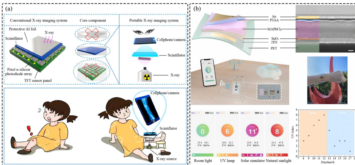
Fig. 19 Schematic diagrams of flexible photodetectors and their application demonstrations in (a) portable X-ray detecting [182] and (b) ultraviolet irradiation monitoring [155]. Reprinted with permission from Ref. [182], copyright@2022, American Chemical Society. Reprinted with permission from Ref. [155], copyright@2022, Elsevier.
