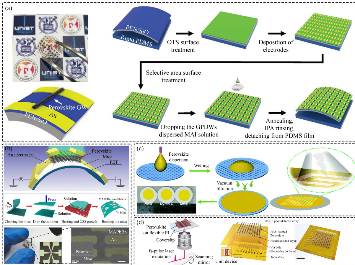
Fig. 6 Perovskite photodetectors on polymer substrates of (a) polyethylenaphthalate (PEN) [75], (b) polyethylene terephthalate (PET) [76], (c) polyvinylidene fluoride (PVDF) [77], and (d) polyimide (PI) [78]. Reprinted with permission from Ref. [75], copyright@2017, Wiley-VCH. Reprinted with permission from Ref. [76], copyright@2020, American Chemical Society. Reprinted with permission from Ref. [77], copyright@2019, Royal Society of Chemistry. Reprinted with permission from Ref. [78], copyright@2020, American Chemical Society.
