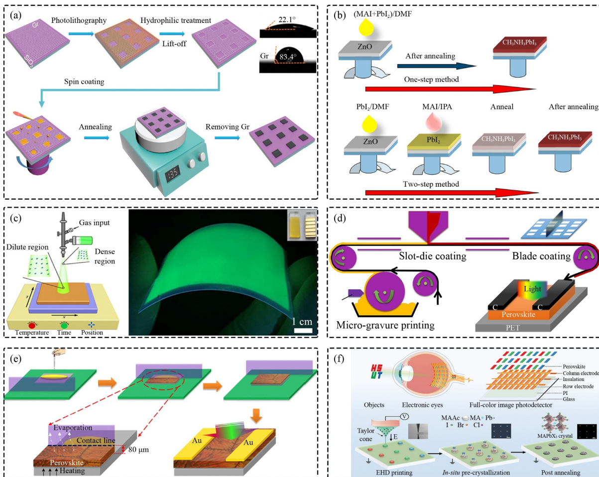
Fig. 2 Solution-based methods of (a) one-step spin coating [25], (b) multiple-step spin coating [26], (c) spray coating [27], (d) slot-die coating [28], (e) blade coating [29], and (f) ink-jet printing [30]. Reprinted with permission from Ref. [25], copyright@2019, Wiley-VCH. Reprinted with permission from Ref. [26], copyright@2020, Elsevier. Reprinted with permission from Ref. [27], copyright@2018, American Chemical Society. Reprinted with permission from Ref. [28], copyright@2019, Elsevier. Reprinted with permission from Ref. [29], copyright@2017, Elsevier. Reprinted with permission from Ref. [30], copyright@2021, Wiley-VCH.
