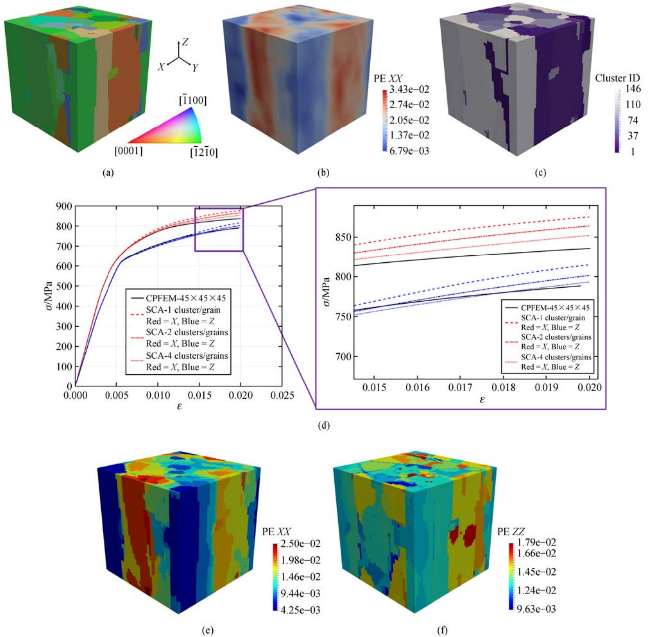
Fig. 9 (a) Synthetically generated columnar microstructure; (b) offline data: Plastic strain; (c) clustering results; (d) overall response and comparison to a DNS simulation with FEA; (e, f) contours of plastic strain in directions X and Z on the surface of the microstructural element as computed with SCA
