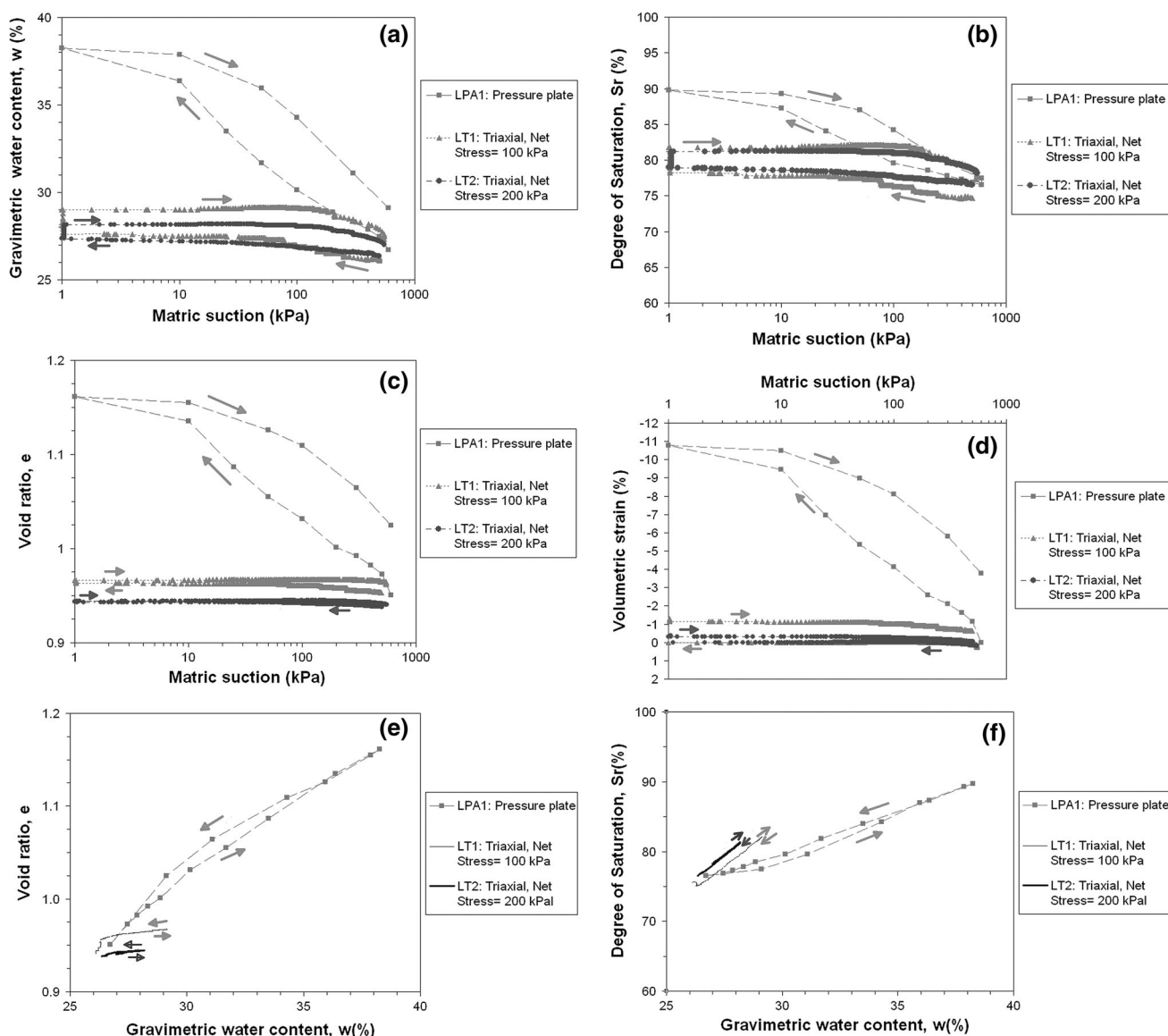
Fig. 6 Effect of net stress; a gravimetric water content versus matric suction relationship; b degree of saturation versus matric suction relationship; c void ratio versus matric suction relationship; d volumetric strain with matric suction change; e void ratio versus gravimetric water content relationship; f degree of saturation versus gravimetric water content relationship
