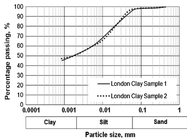
Fig. 1 Particle size distribution of the London Clay
