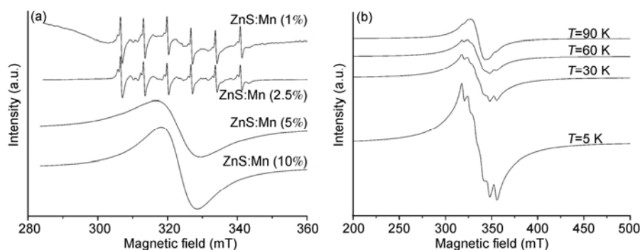
Figure 1 Room temperature ESR spectra of ZnS:Mn (a) and low temperature ESR spectra of ZnS:Mn (20%) (b).
