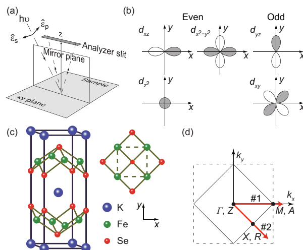
Figure 1 (Color online) (a) Experimental setup for polarization-dependent ARPES. (b) Illustration of the spatial symmetry of the 3d orbital with respect to the xz plane. (c) The schematic crystal structure of K_x\text{Fe}_{2-y}\text{Se}_2 superconductor. The right side is the top view of the FeSe trilayer, and the x and y axes are along the two Fe-Fe bond directions. (d) Two-dimensional projection of the Brillouin zone (solid line) and the unfolded Brillouin zone (dashed line) [23].
