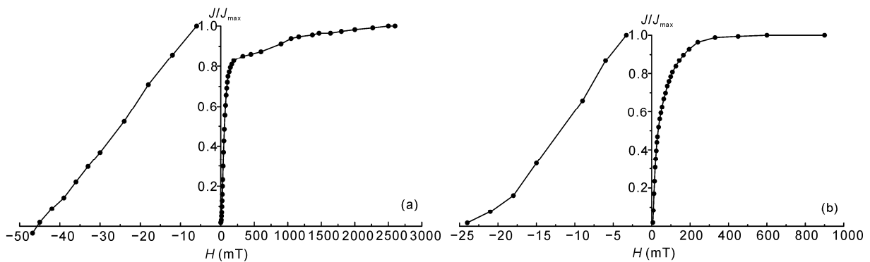
Figure 3 SIRM acquisition curves and Remanent coercivity spectra for (a) Wanning diabase; (b) Wanning gabbro.
