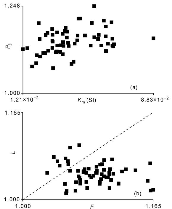
Figure 7 (a) Degree of magnetic anisotropy ( P_j ) versus mean susceptibility ( K_m ) for the Wanning gabbro; (b) Flinn plot of the magnetic fabric of the Wanning gabbro.
