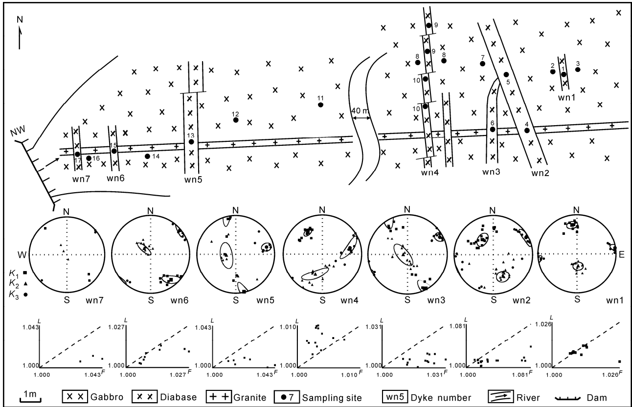
Figure 2 Sampling sites, AMS projections, and Flinn plots of 7 diabase dykes at Wanning (in geographic coordinates).
