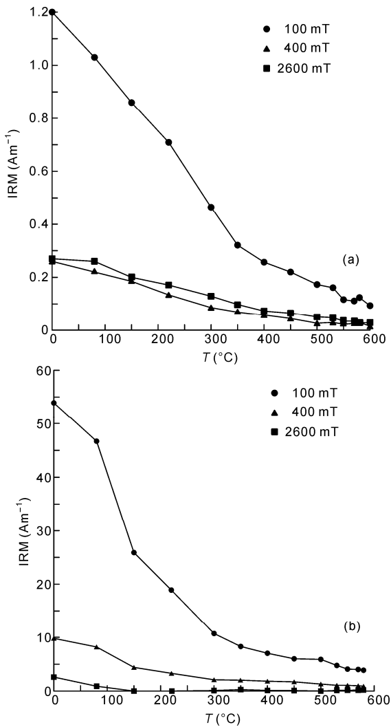
Figure 4 Triaxial IRM thermal demagnetization curves. (a) Wanning diabase; (b) Wanning gabbro.
