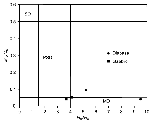
Figure 5 Day plot of magnetic grain-sizes for the Wanning gabbro and diabase dykes.
