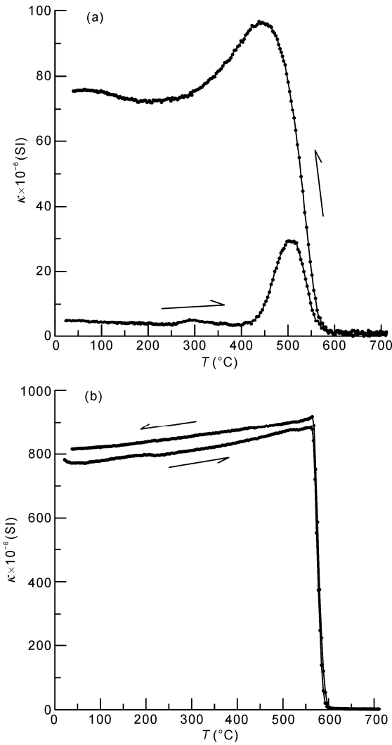
Figure 6 Thermomagnetic curves under argon atmosphere. (a) Wanning diabase; (b) Wanning gabbro.
