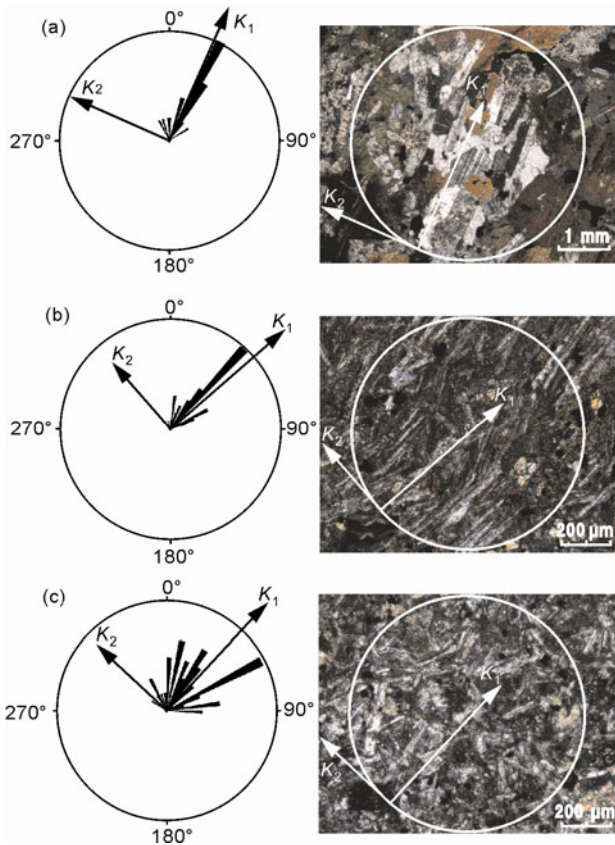
Figure 10 Oriented thin-sections in the magnetic foliation plane ( K_1 - K_2 ) and rose diagrams of plagioclase phenocrysts contrasted with K_1 . (a) Wanning gabbro; (b), (c) Wanning diabase.
