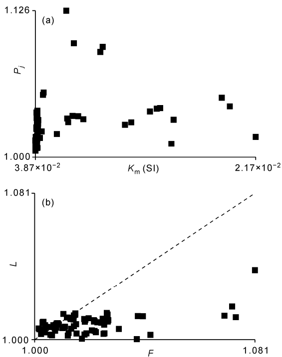
Figure 9 (a) Degree of magnetic anisotropy ( P_j ) versus mean susceptibility ( K_m ) for the Wanning diabase; (b) Flinn plot of the magnetic fabric of the Wanning diabase.
