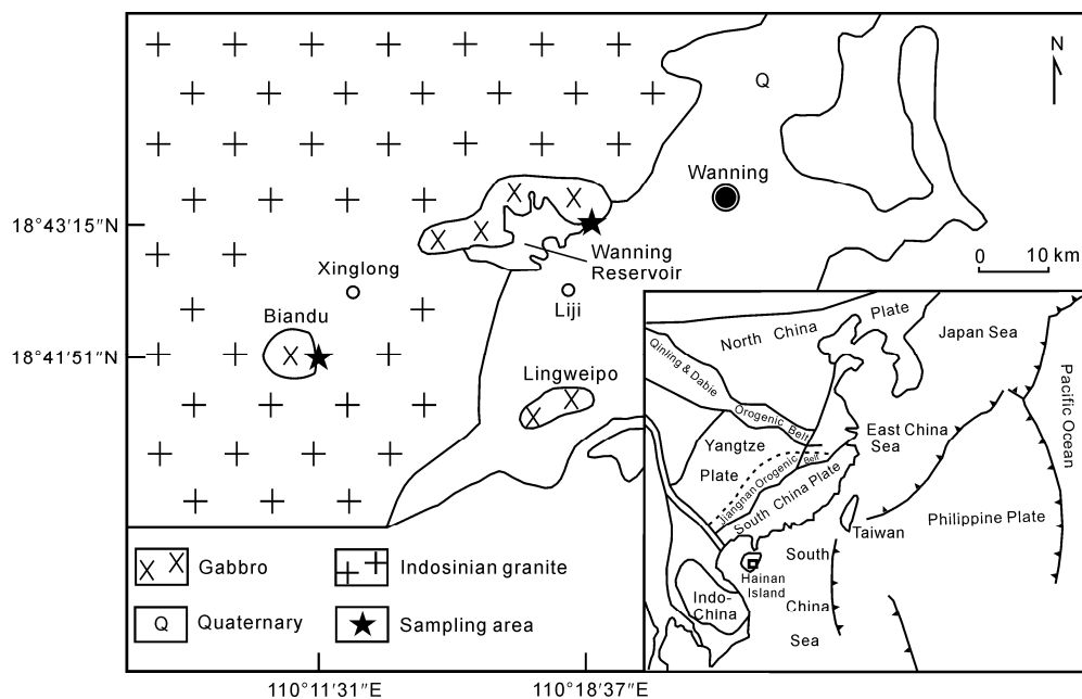
Figure 1 Geological sketch map of Hainan Island and the sampling area.
