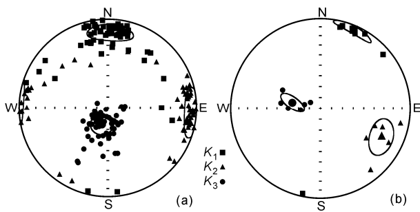
Figure 8 Equal-area projections of AMS in geographic coordinates. (a) Wanning gabbro; (b) Biandu gabbro.
