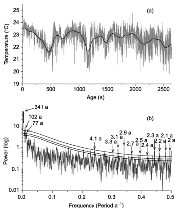
Figure 1 Stalagmite record of warm-season temperatures for the past 2650 years in Beijing with spectral features added. (a) Original warm-season temperature reconstruction (gray line) [2] with the thick line representing non-linear and low frequency trends (the first principle component, PC1). The top of the record corresponds to 1985 AD. (b) Multi-taper spectrum of the warm-season temperature time-series. The three horizontal lines indicate the 99%, 95% and 90% confidence limits, respectively.
