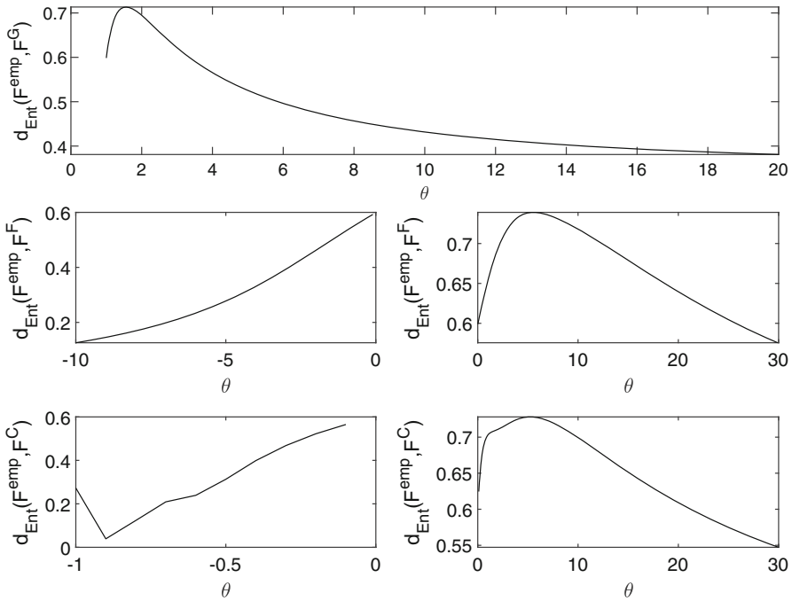
Fig. 8 Distance d_{Ent}(F_S^{\text{emp}}, F_S^C) , when C = C_G in (7) (upper figure), C = C_F in (8) (middle figure) and C = C_C in (9) (lower figure). Also in this case, the two panels in the middle and lower figures are taken as distinct entities to emphasize the domain of the related parameters
