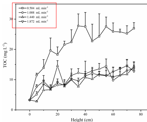
Fig. 3 The concentrations of total organic carbon (TOC) along the height of the up-flow bioreactor (UFBR)
