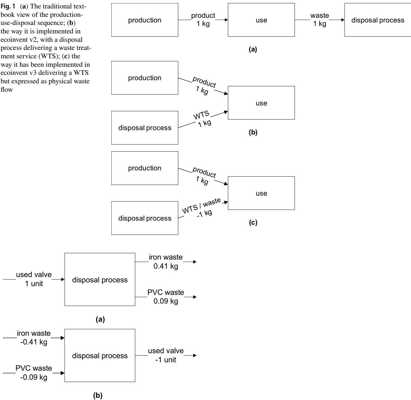
Fig. 2 (a) The traditional textbook view of a particular disposal process that transforms a waste into materials; (b) the way this process is implemented in ecoinvent v3
