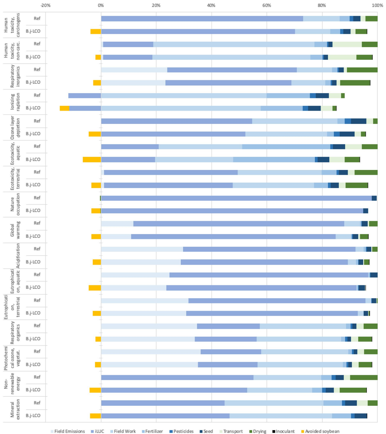
Fig. 3 Contribution analysis of the impacts of soybean production with ( B,j-LCO ) and without ( Ref ) the inoculant. A negative contribution means a reduction of the impact. The field effect includes impacts from (in blue): field emissions, iLUC, field work, fertilizers, pesticides and seeds; the downstream effect includes impacts from (in green) transport and drying; the yield effect includes impacts from the avoided soybean (in yellow) and the upstream effect includes impacts from the inoculant (in black)
