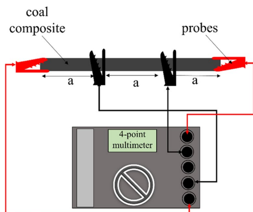
Fig. 4 Arrangement of the four-point probe resistance measurement of the carbon/ceramic composites
