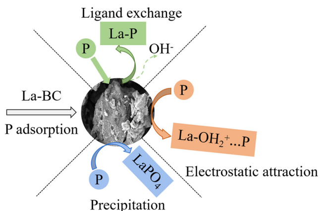
Fig. 9 A schematic diagram for the mechanism of phosphate adsorption on La-BC
