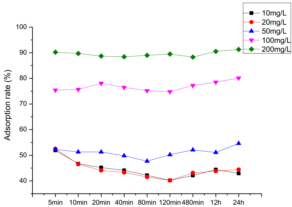
Figure S3. The curve of the rate of As adsorption by different concentration of zinc oxide nanoparticles.
