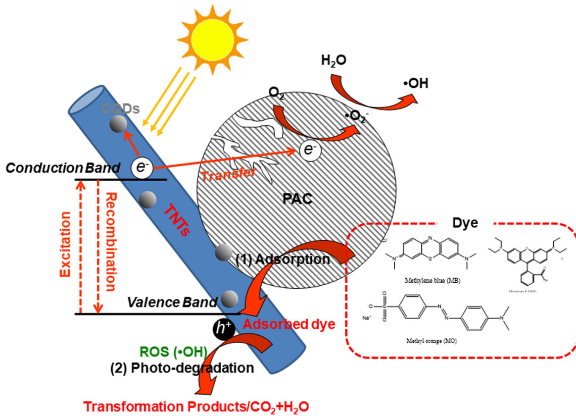
Fig. 8 Schematic of a two-step adsorption-photodegradation process for complete destruction of dyes by TNTs@PAC (modified from Liu et al., 2016)
