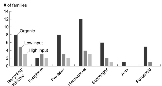
Fig. 4 Functional roles represented by insect families positively correlated with organic and low- and high-input farms for both pitfall and yellow bowl traps, as displayed in Fig. 3
