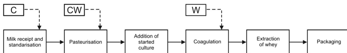
Fig. 2 Flow diagram for processes occurring at a cheese plant where C cleaning and sanitization solutions, CW cooling water, W water wash
