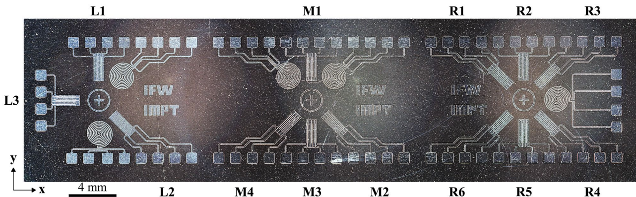
Fig. 3 Directly deposited strain gauges and temperature sensors with an insulation layer on stainless steel. The strain gauges are named according to their belonging to the sensor layout L, M or R (L=Left, M=Middle, R=Right)
