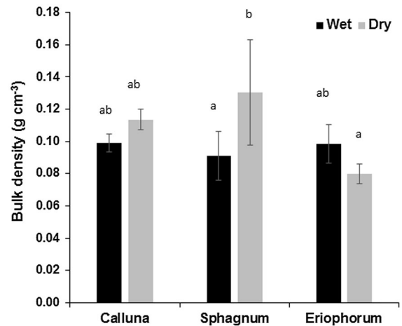
Fig. 4 Mean bulk densities ( \pm 95% confidence interval) of the top 5 cm of peat for wet (0 cm water table depth; WTD) and dry ( -35 cm WTD) cores after 9 months of constant WTD in the laboratory trial for the different vegetation groups ( Calluna , Sphagnum or Eriophorum dominated surface vegetation cover). Significant differences (ANOVA) are indicated by different letters
