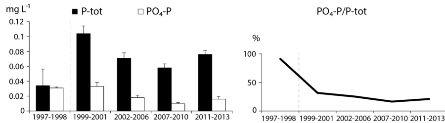
Fig. 4 Concentrations of total phosphorus ( P_{\text{tot}} ) and phosphate-P ( \text{PO}_4\text{-P} ) in Västskär wetland, 1997–2013. Left Mean values for the sub-areas and periods. Right ratio of \text{PO}_4\text{-P} to P_{\text{tot}}
