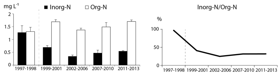
Fig. 3 Inorganic ( N_{\text{inorg}} ) and organic ( N_{\text{org}} ) nitrogen concentrations in Västskär wetland, 1997–2013. Left Mean values for sub-areas and periods. Right ratio of N_{\text{inorg}} to N_{\text{org}}
