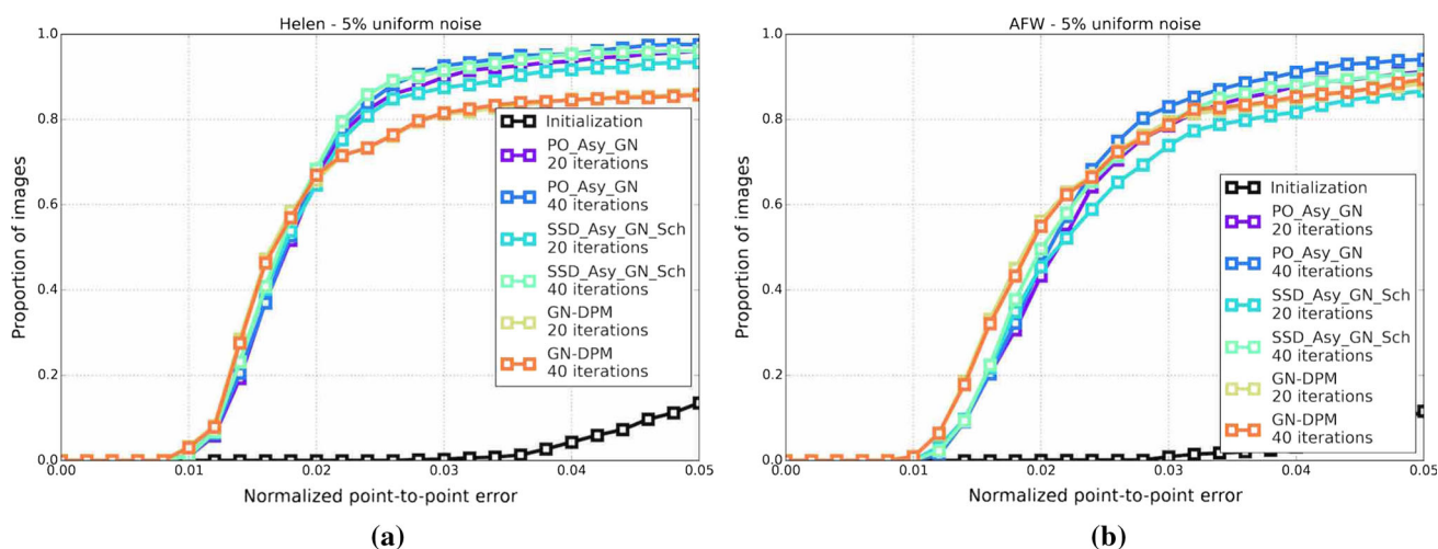
Fig. 14 Results showing the fitting accuracy of the SSD and Project-Out Asymmetric Gauss-Newton algorithms on the Helen and AFW databases. a CED on the Helen test dataset for the Project-Out and
