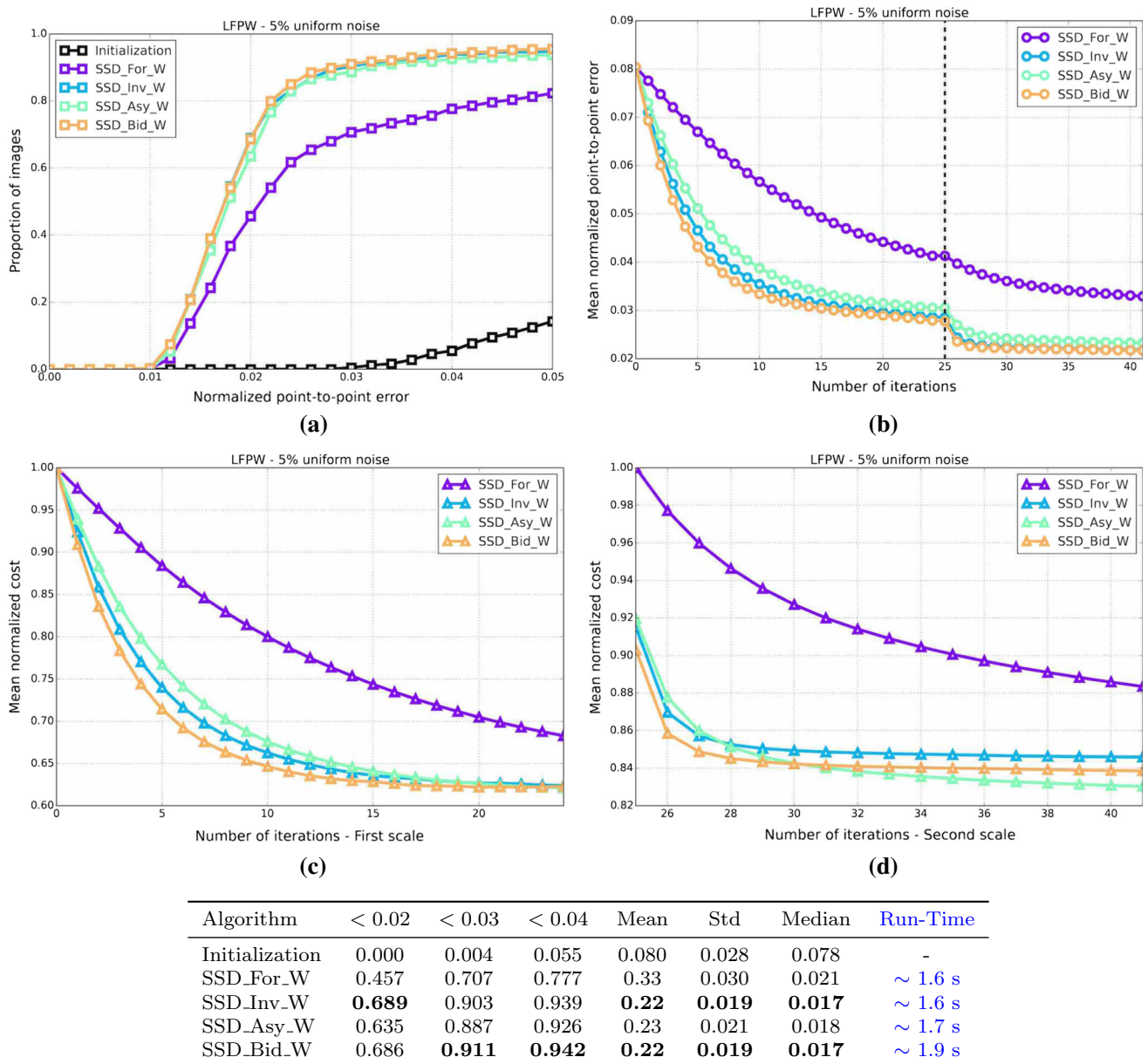
Fig. 7 Results showing the fitting accuracy and convergence properties of the SSD Wiberg algorithms on the LFPW test dataset. a CED on the LFPW test dataset for all SSD Wiberg algorithms initialized with 5% uniform noise. b Mean normalized point-to-point error versus number of iterations on the LFPW test dataset for all SSD Wiberg algorithms initialized with 5% uniform noise. c Mean normalized cost versus number of first scale iterations on the LFPW test dataset for all SSD Wiberg algorithms initialized with 5% uniform noise. d Mean normalized cost versus number of second scale iterations on the LFPW test dataset for all SSD Wiberg algorithms initialized with 5% uniform noise. e Table showing the proportion of images fitted with a normalized point-to-point error below 0.02, 0.03 and 0.04 together with the normalized point-to-point error mean, std and median for all SSD Wiberg algorithms initialized with 5% uniform noise
