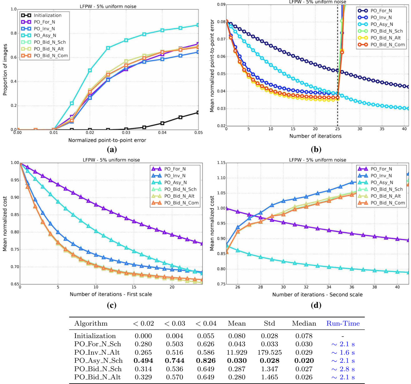
Fig. 9 Results showing the fitting accuracy and convergence properties of the Project-Out Newton algorithms on the LFPW test dataset. a CED graph on the LFPW test dataset for all Project-Out Newton algorithms initialized with 5% uniform noise. b Mean normalized point-to-point error versus number of iterations on the LFPW test dataset for all Project-Out Newton algorithms initialized with 5% uniform noise. c Mean normalized cost versus number of first scale iterations on the LFPW test dataset for all Project-Out Newton algorithms initialized
