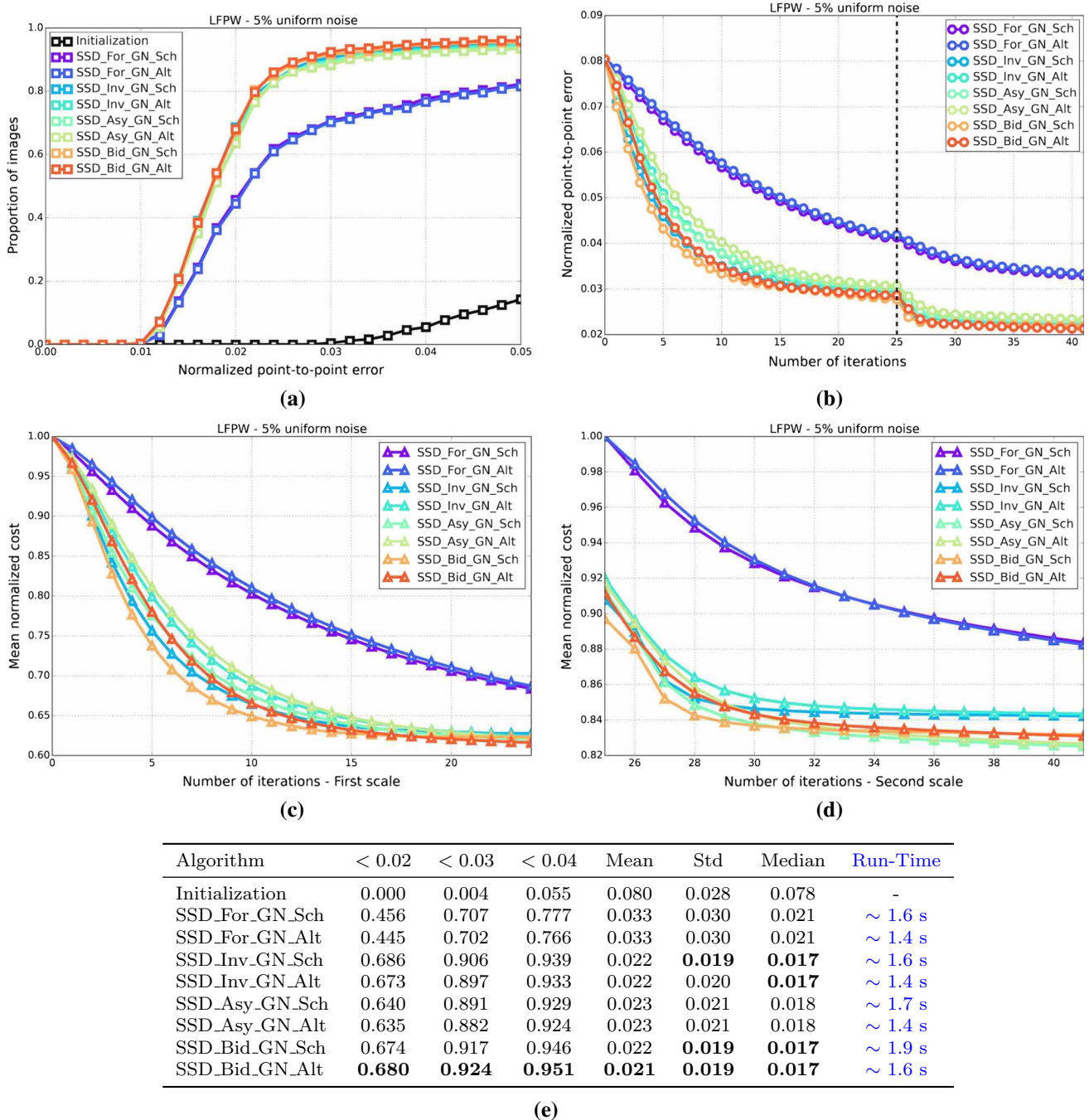
Fig. 5 Results showing the fitting accuracy and convergence properties of the SSD Gauss-Newton algorithms on the LFPW test dataset initialized with 5% uniform noise. a CED on the LFPW test dataset for all SSD Gauss-Newton algorithms initialized with 5% uniform noise. b Mean normalized point-to-point error versus number of iterations on the LFPW test dataset for all SSD Gauss-Newton algorithms initialized with 5% uniform noise. c Mean normalized cost versus number of first scale iterations on the LFPW test dataset for all SSD Gauss-Newton
