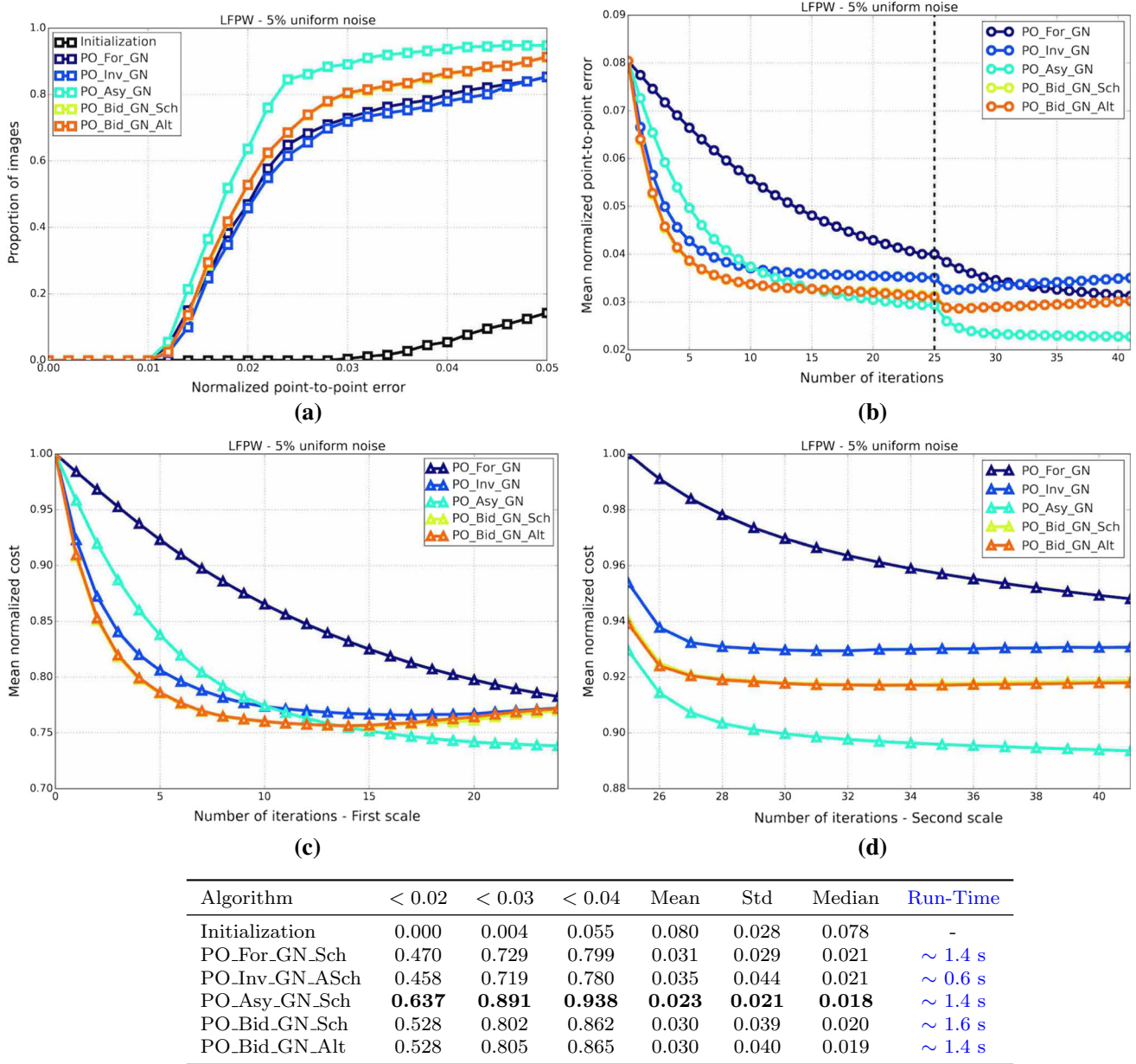
Fig. 8 Results showing the fitting accuracy and convergence properties of the Project-Out Gauss-Newton algorithms on the LFPW test dataset. a CED graph on the LFPW test dataset for all Project-Out Gauss-Newton algorithms initialized with 5% uniform noise. b Mean normalized point-to-point error versus number of iterations on the LFPW test dataset for all Project-Out Gauss-Newton algorithms initialized with 5% uniform noise. c Mean normalized cost versus number of first scale iterations on the LFPW test dataset for all Project-Out
