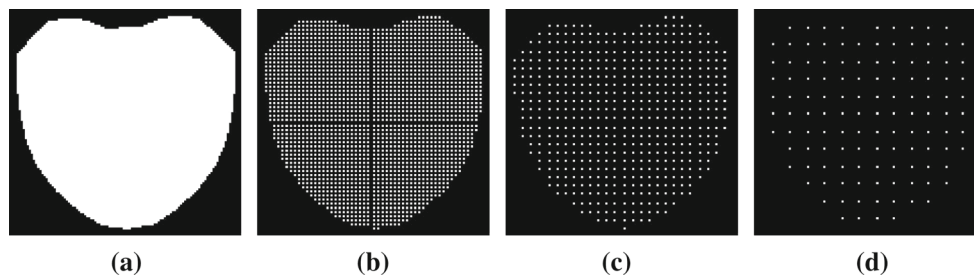
Fig. 3 Subset of pixels on the reference frame used to optimize the SSD and Project-Out cost functions for different sampling rates. a 100 %, b 50 %, c 25 %, d 12 %
