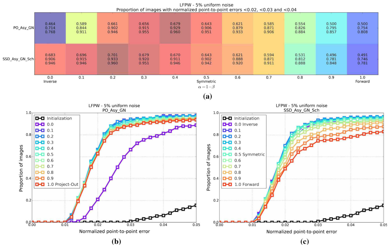
Fig. 12 Results quantifying the effect of varying the value of the parameters \alpha = 1 - \beta in Asymmetric algorithms. a Proportion of images with normalized point-to-point errors smaller than 0.02, 0.03 and 0.04 for the Project-Out and SSD Asymmetric Gauss-Newton algorithms for different values of \alpha = 1 - \beta and initialized with 5% noise. Colors encode overall fitting accuracy, from highest to lowest: red, orange, yellow, green, blue and purple. b CED on the LFPW test dataset for Project-Out Asymmetric Gauss-Newton algorithm for different values of \alpha = 1 - \beta and initialized with 5% noise. c CED on the LFPW test dataset for the the SSD Asymmetric Gauss-Newton algorithm for different values of \alpha = 1 - \beta and initialized with 5% noise (Color figure online)
