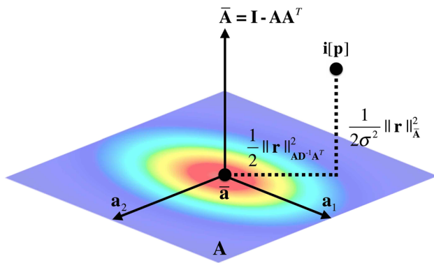
Fig. 2 The fits AAMs by minimizing two different distances: (i) the Mahalanobis distance within the linear appearance subspace; and (ii) the Euclidean distance to the linear appearance subspace (i.e. the Euclidean distance within its orthogonal complement) weighted by the inverse of the estimated image noise
