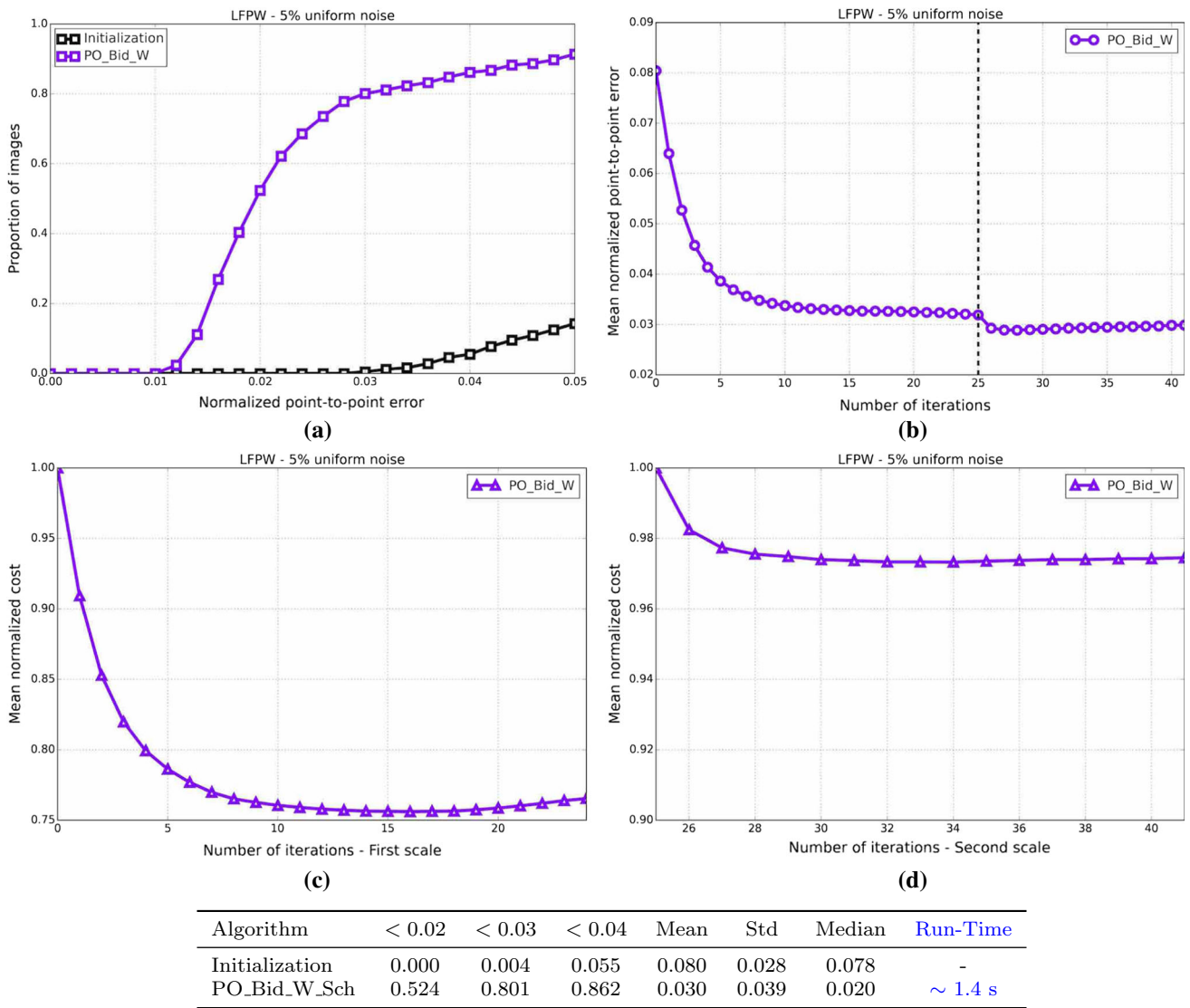
Fig. 10 Results showing the fitting accuracy and convergence properties of the Project-Out Wiberg algorithms on the LFPW test dataset. a Cumulative Error Distribution graph on the LFPW test dataset for all Project-Out Wiberg algorithms initialized with 5% uniform noise. b Mean normalized point-to-point error versus number of iterations graph on the LFPW test dataset for all Project-Out Wiberg algorithms initialized with 5% uniform noise. c Mean normalized cost versus number of first scale iterations graph on the LFPW test dataset for all Project-Out
