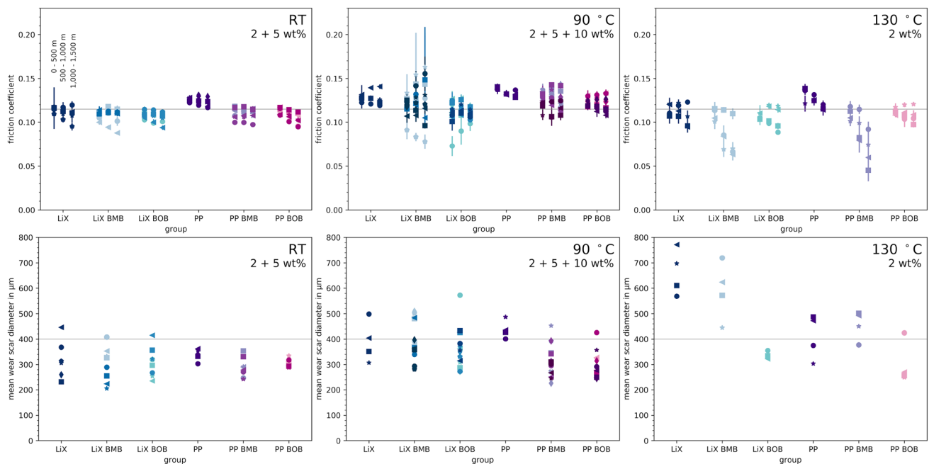
Fig. 3 Friction (top) and wear (bottom) results of pin-on-disk test series POD RT, POD 90, and POD 130 for [P_{6,6,6,14}][BMB] and [P_{6,6,6,14}][BOB] in the same manner as Fig. 2. The data for the neat
