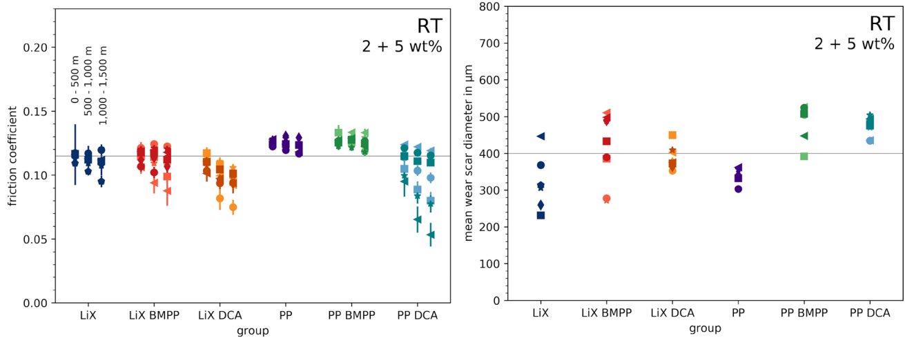
Fig. 2 Friction (left) and wear (right) results of pin-on-disk test series POD RT for [P_{6,6,6,14}][DCA] and [P_{6,6,6,14}][BMPP] additives. For the friction plots, each data point represents the average friction coefficient within a sliding distance range of either 0–500 m, 500–1 000 m, or 1 000–1 500 m (from left to right for each group). The error bars indicate the standard deviation of the friction coefficient within the
