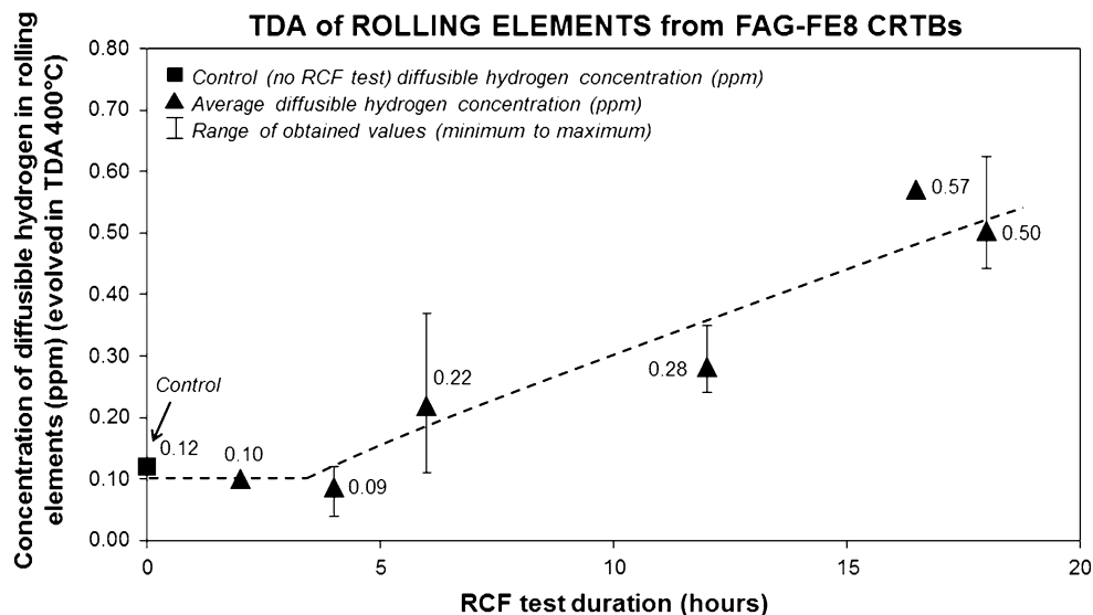
Fig. 3 Average concentrations of diffusible hydrogen measured by TDA at \leq 400 °C using set-up #1 in the rolling elements post-RCF testing. See Table 2 for individual hydrogen TDA measurements
