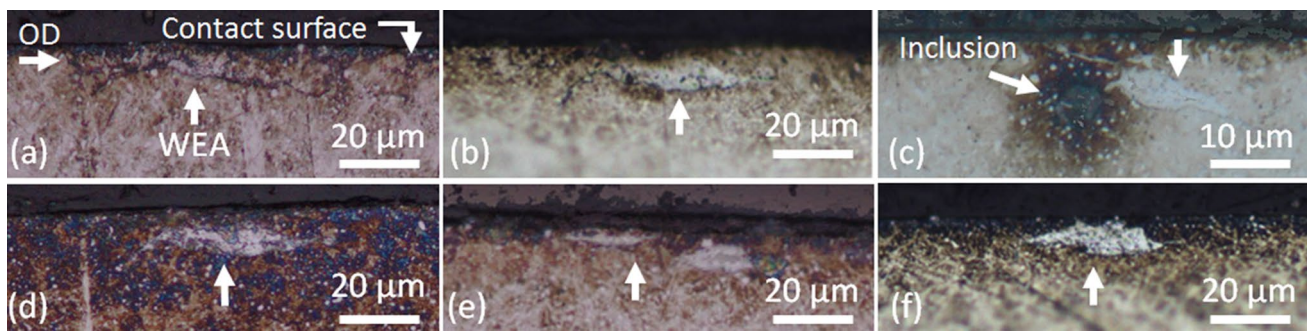
Fig. 7 Optical images of typical 18-h near-surface WEA/WEC features (a–f). Over-rolling direction (OD) left to right
