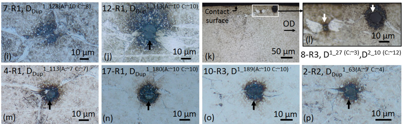
Fig. 9 Images of typical inclusion–WEC interactions recorded at 6 and 18 h. Images a–d show the location of the inclusion–WEC interactions from SEM images e–h , respectively, at 6 h. Images i–p are optical images of typical inclusion–WEC interactions recorded at 18 h. k and l show an example of a butterfly WEC with correspond-
