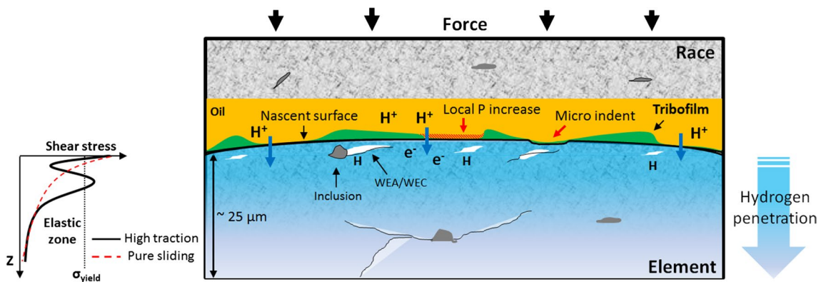
Fig. 15 Hypothesised mechanisms of near-surface ( < 25 \mu\text{m} ) WEA/WECs formation. H^+ denotes molecular hydrogen, H denoting monoatomic hydrogen diffused into the bearing steel. e^- denotes free elec-
