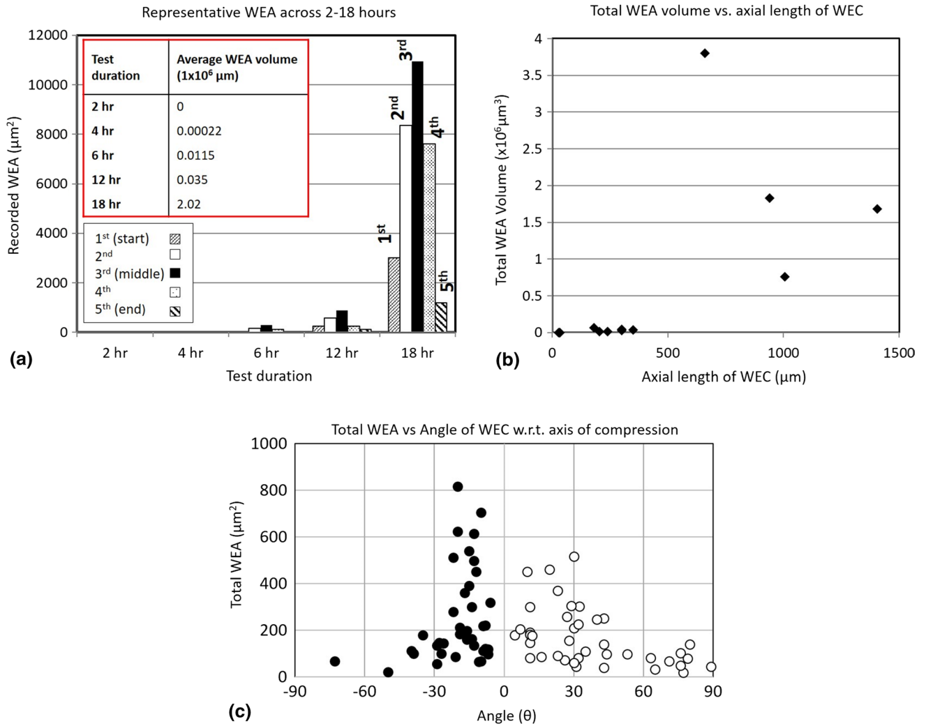
Fig. 14 WEA volume and area analysis. a Representative average WEA across 2–18 h. b Total WEA volume versus axial length of WEC. c Total WEA measured vs the respective angle of the WEC for 5 different randomly chosen WECs at 18 h
