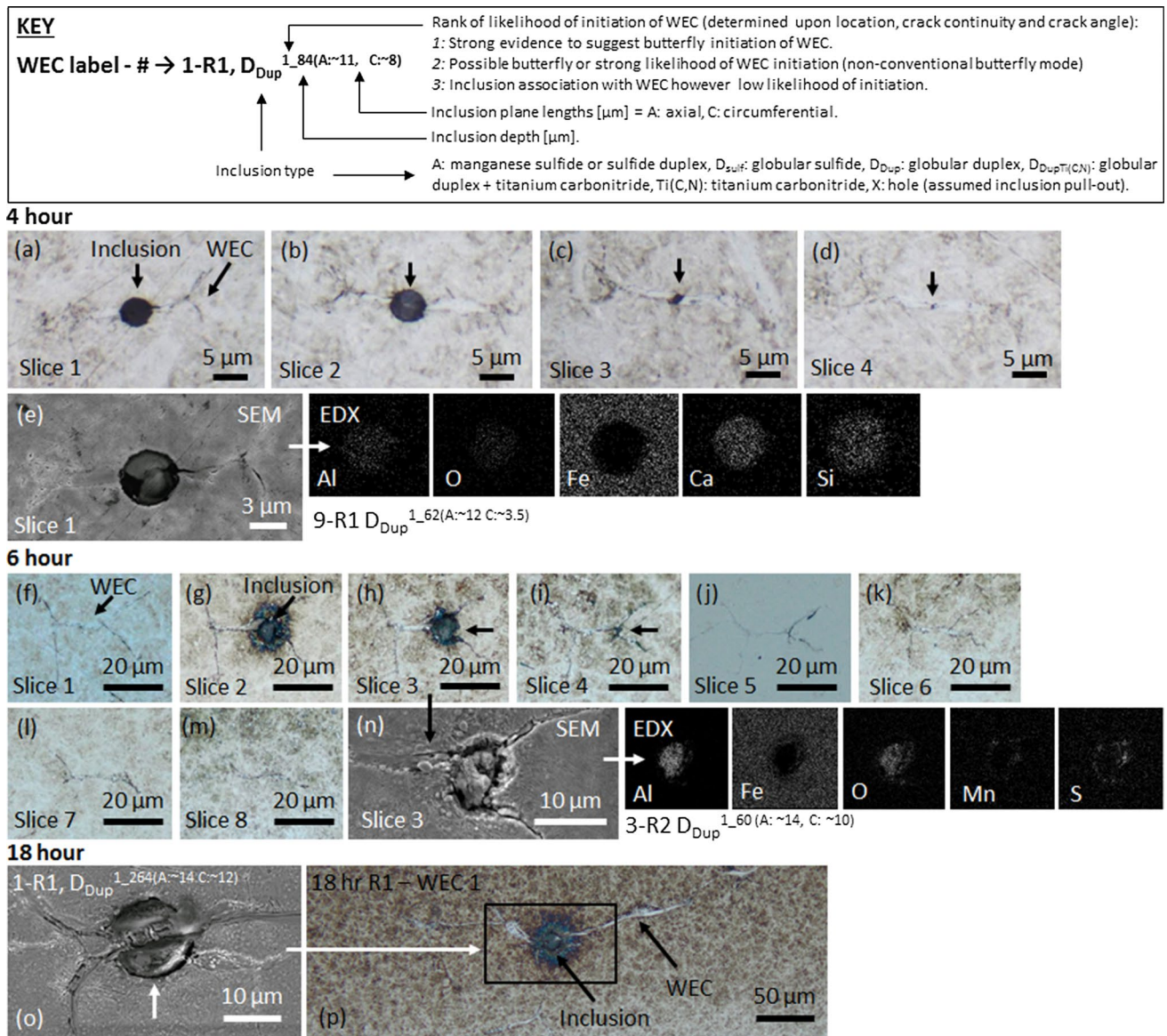
Fig. 8 Optical images of mapped WECs and inclusion–WEC interactions at 4, 6 and 18 h. a–d represent the individual slices from start (slice 1) to finish (slice 4) of mapped 4-h WEC-9 R1. SEM image, e shows inclusion–WEC interaction from (a) slice 1 with corresponding EDX chemical maps. f–m Mapped 6-h WEC-3 R2, images ( f–m ) represent the individual slice images from start (slice 1) to near finish (slice 8). Images g–i show the location of the inclusion–WEC interac-
