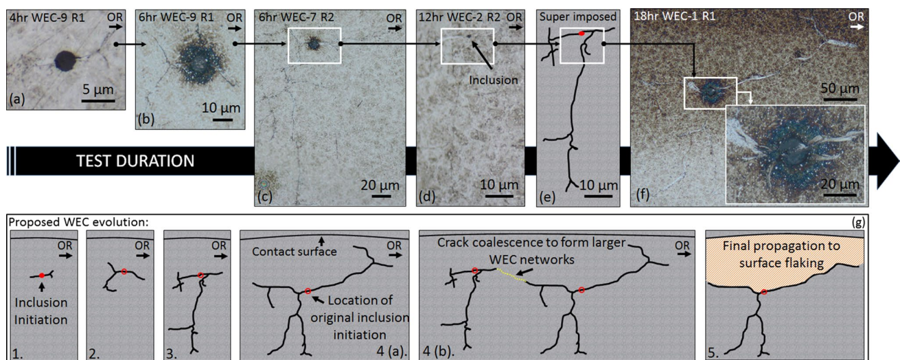
Fig. 16 Optical images of WECs recorded at 4–18 h. a–f show examples of typical WECs recorded between 4 and 18 h. e Super-imposed image of the 12-h WEC shown in (d) , the inclusion highlighted in red. g Proposed stages of WEC evolution; (1) initiation via inclusion in the subsurface, (2) propagation into ‘star-like’ WEC (see
