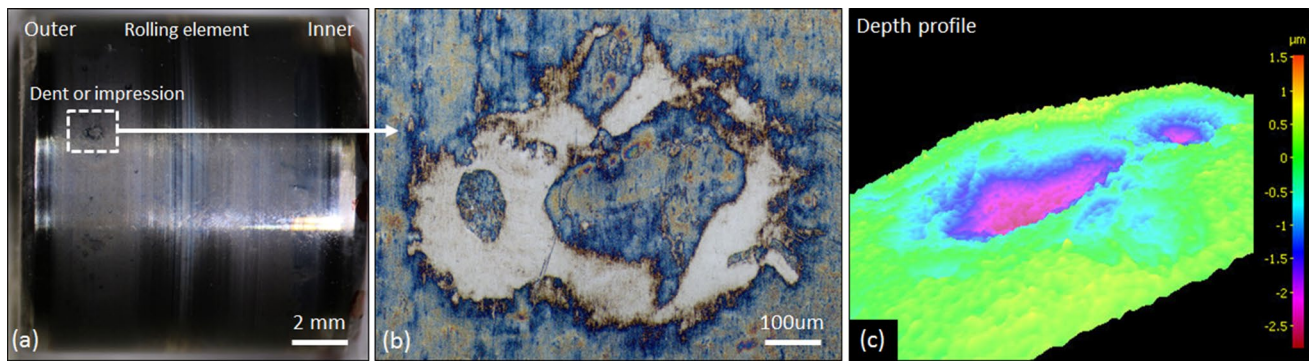
Fig. 4 Surface analysis of a typical indent found on the 18-h rollers. a Optical macroimage of roller indicating location of indent on the contact surface. b Magnified optical image of the indent. c Depth profile analysis of the indent
