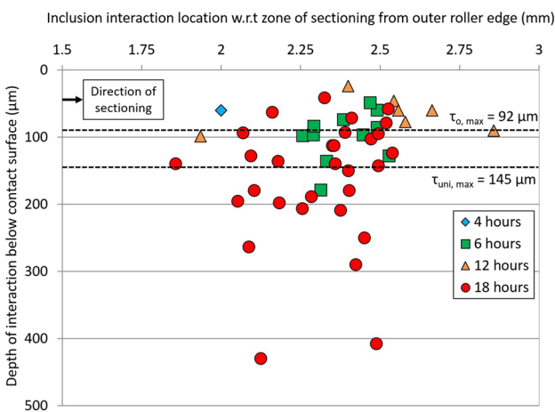
Fig. 10 a Spatial distribution and depth of inclusion–WEC interactions w.r.t the depth of maximum subsurface shear stresses judged to have a high likelihood of crack initiation (rank 1 or 2). See Fig. 8 and ‘Appendix B’ for more information on the inclusion ranking system
