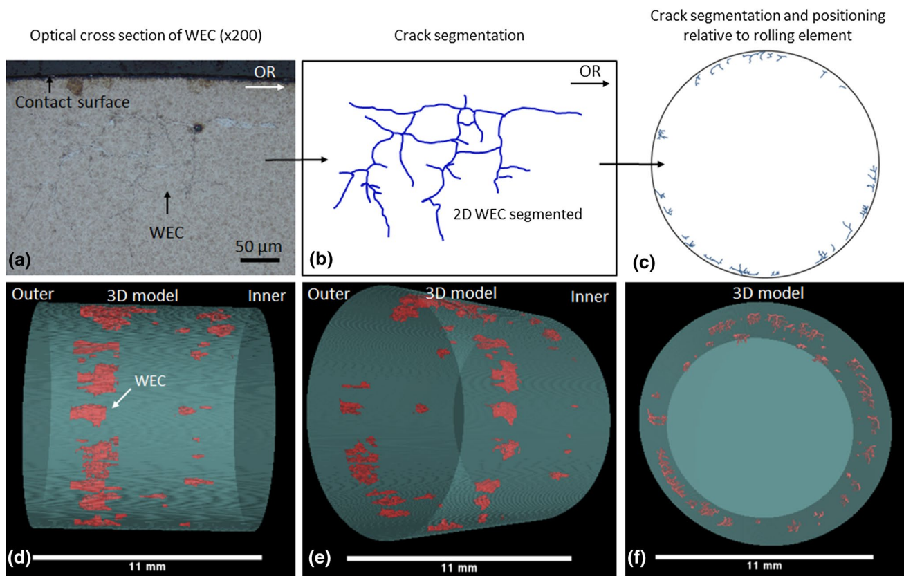
Fig. 11 3D model of total WEC damage recorded across 18-h R1. a Optical cross-sectional image of a WEC. b 2D segmentation of WEC from optical image in (a) . c Placement of 2D segmented WEC into its
