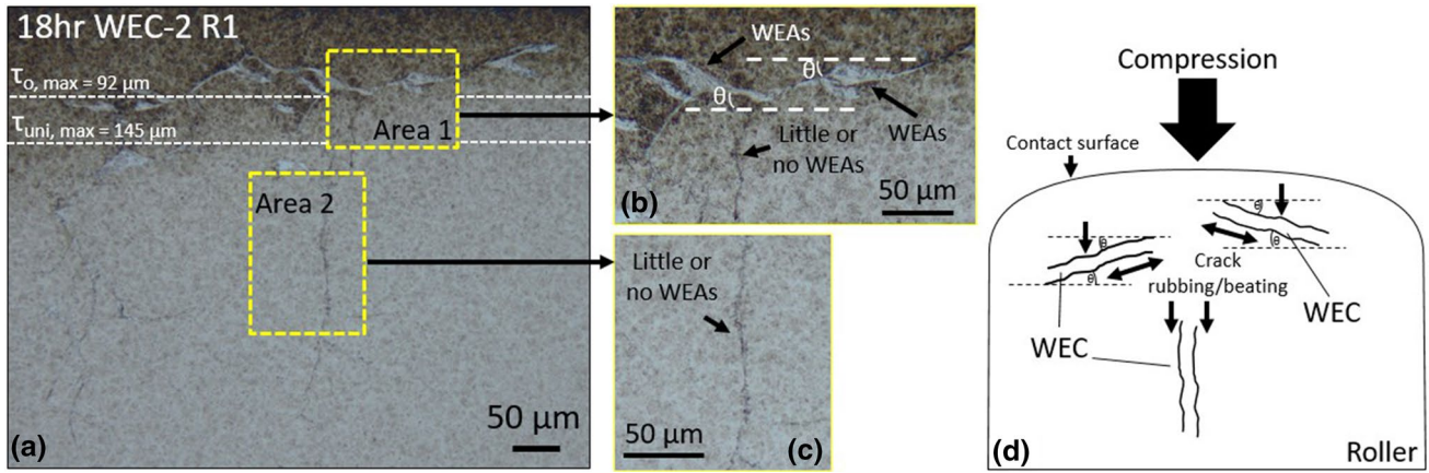
Fig. 17 Optical image of a WEC demonstrating the influence of crack angle w.r.t the axis of compression and depth of maximum subsurface shear stresses ( \tau_{o, \max} = 92 \mu\text{m} , \tau_{uni, \max} = 145 \mu\text{m} ) on the formation of WEAs. a Areas 1 and 2 show two different orientations of crack propagation, Area 1 shows cracks at an angle \theta to the axis of compression along with a vertical crack parallel to the compression axis,
