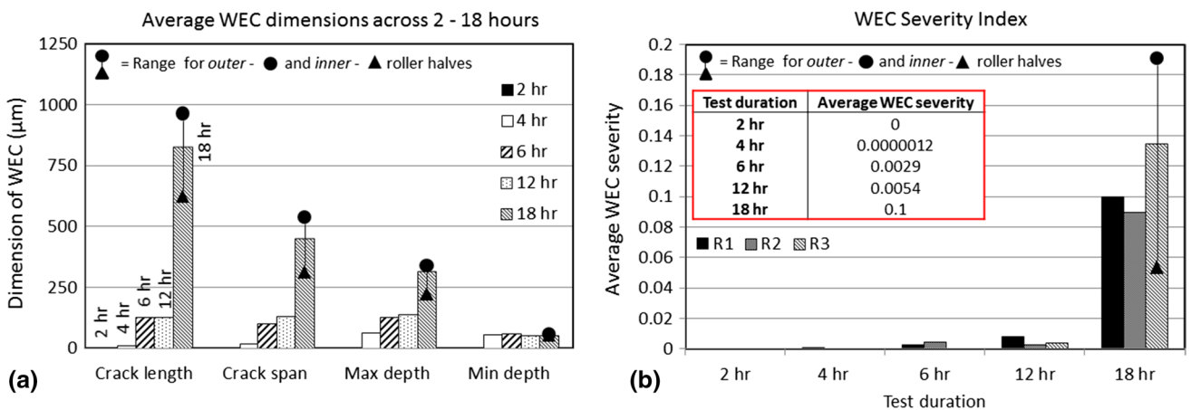
Fig. 13 a Average WEC dimensions in the rollers across 2–18-h tests, see ‘Appendix C’ for details on measurement of relevant crack dimensions. b WEC severity index in the rollers for the 2–18-h tests
