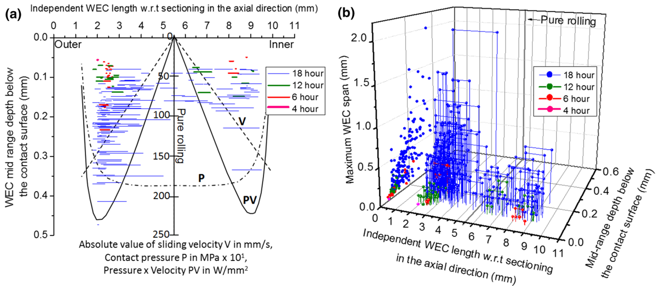
Fig. 12 a Distribution of individual WECs recorded in 4–18-h rollers across the entire axial length (x-axis) of rollers from outer to inner edge and corresponding mid-range depth below the contact surface (0.00 mm) (y-axis). Pressure P, absolute sliding velocity V and slip energy PV are also represented (adapted from [49]). b 3D plot of all independently recorded WECs across 4–18 h. X-axis represents the
