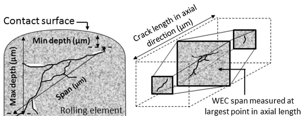
Fig. 19 Schematic illustrating the measurements of WEC dimensions
