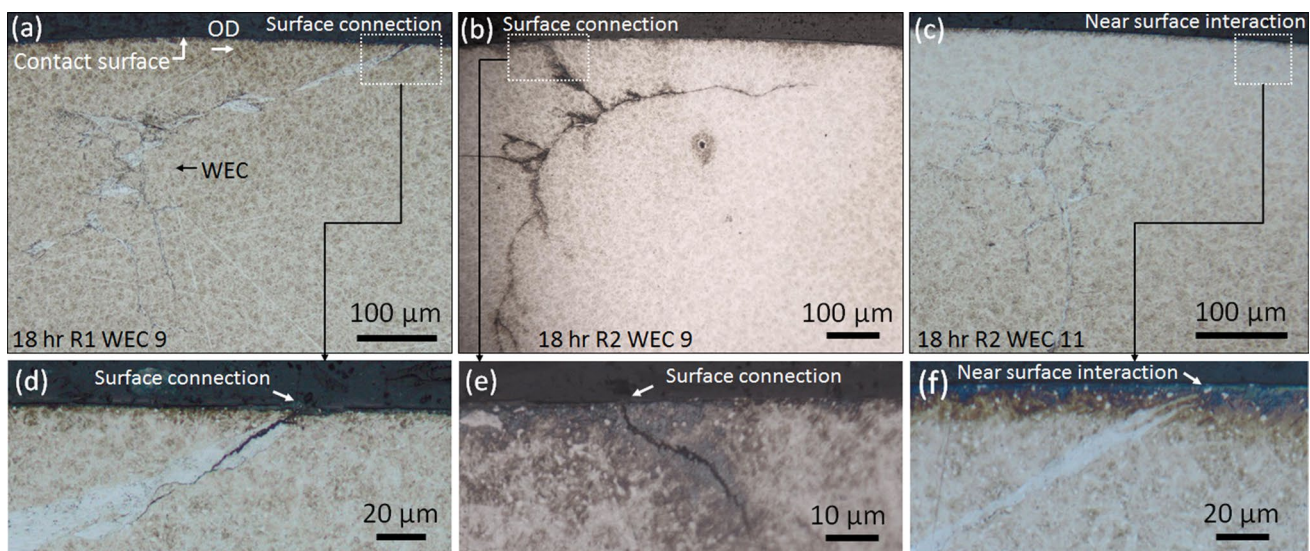
Fig. 6 Optical images of 18-h surface connections and near-surface interactions. a WEC-9 R1 surface connection, surface connection length in axial sectioning direction < 30 \mu\text{m} . b WEC-9 R2 surface connection, surface connection length \sim 500 \mu\text{m} . c WEC-11 R2 near-
