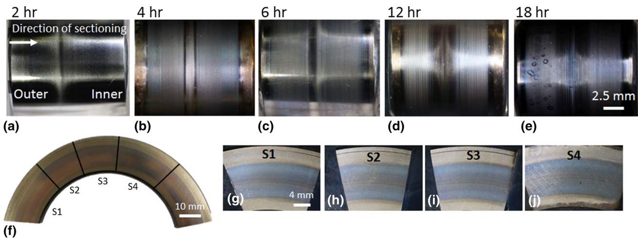
Fig. 5 Optical microscope images of a single roller from each RCF test duration (2–18 h) and 18-h raceway sections chosen for subsequent sectioning. Images g–j are optical macroimages of the corresponding sections (S1–S4) shown in f . S denotes sample number
