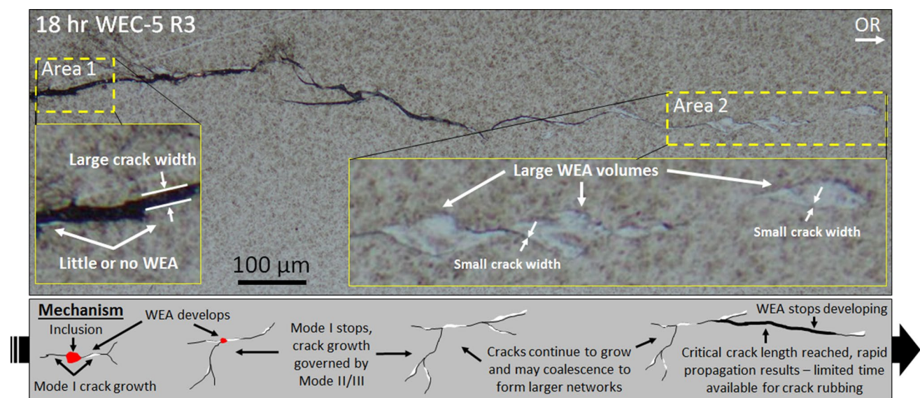
Fig. 18 Optical image of a WEC demonstrating the influence of crack width on the generation of WEAs. Area 1 shows a large crack width, and Area 2 shows a small crack width, with respective magni-
