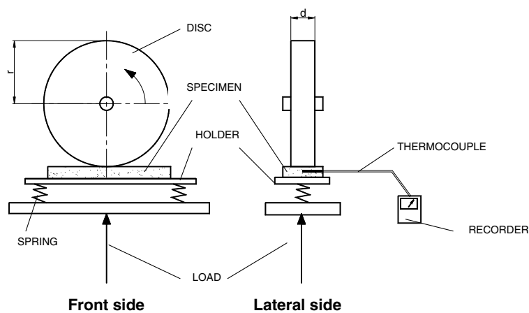
Figure 1. Schematic presentation of the disc-on block type wear test apparatus.
