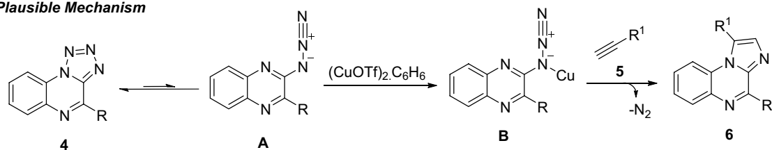
Scheme 2 Reaction tetrazoloquinoxalines 4 with alkynes 5 to synthesize imidazo[1,2- a ]quinoxalines 6 via copper(I) triflate catalyzed denitrogenative annulation
