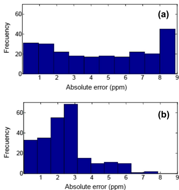
Fig. 8 Histograms of the absolute error and the frequency of its occurrence during the reaction time, corresponding to a the first (Rv1) and b second (Rv2) catalyst reuses, respectively
