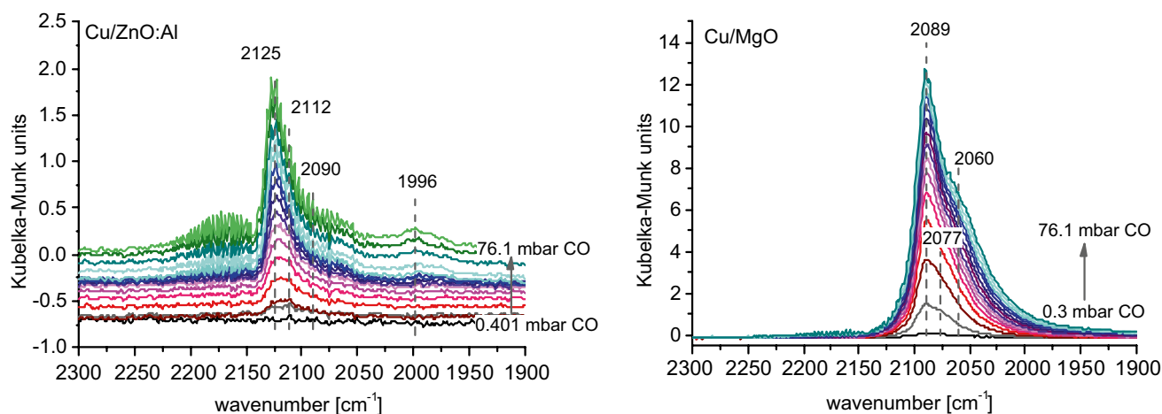
Fig. 2 Infrared spectra of CO adsorbed on the reduced catalysts Cu/ZnO:Al (left) and Cu/MgO (right) after reduction of the catalysts at 523 K in the infrared chamber ( T_{\text{ads}}=300\text{ K} , increasing equilibrium pressures from 0.3 to 76 mbar CO)
