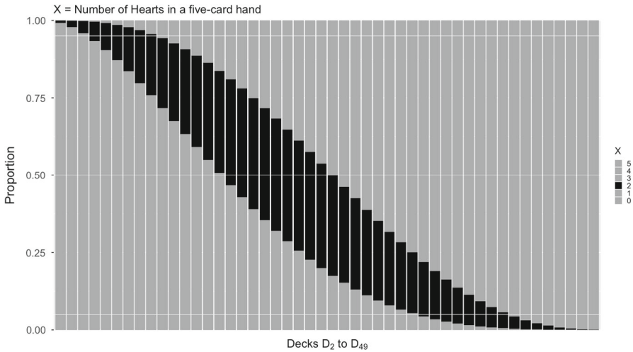
Fig. 1 The left most bar presents the distribution of the number of hearts in five-card hands for D_2 , the deck with 2 hearts. Nearly all the hands have 0 or 1 hearts (the height of gray bar gives the proportion of all such hands) and the remainder of the hands have 2 hearts (height of the black bar gives the proportion). Hands with 3, 4, or 5 hearts are not possible with deck D_2 . The next bars present the corresponding distributions for decks D_3, D_4, \dots, D_{48} , and D_{49} . Each bar consists of 6 segments, one for each possible value of X . Since x = 2 was observed we use only two colors: black to represent the observed value and gray for values that are smaller (0 and 1) or larger (3, 4 or 5). The horizontal line at 0.50 intersects the black bars for decks D_{17} through D_{26} indicating the observed value of 2 hearts is the median and so represents no evidence against these models. The remaining two horizontal lines are at 0.05 and 0.95, the traditional values used to indicate samples sufficiently extreme as to provide significant evidence against the model
