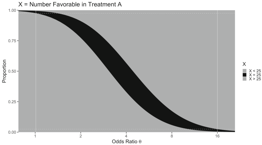
Fig. 2 C_{(x)obs}^{0.05} consists of the models with odds ratio between 1.01 and 16.0. Horizontal dashed white lines are at 0.025 and 0.975. The vertical white line at \theta = 1.01 shows the distribution of X for the model where the odds of success with Treatment A are 1.01 times that of Treatment B and the total number of successes observed is 42. For this model, the observation of 25 favorable responses for Treatment A is in the upper 2.5% of possible values for X making the observation significantly larger than would be expected. Because patients were randomly assigned to treatments, the distribution of X given by the model with odds ratio \theta = 1.01 provides the probability of observing 25 or more favorable responses for treatment A. Vertical lines where \theta > 1.01 show this probability increases for these models. The vertical white line at \theta = 16.0 shows the distribution of X for the model where the odds of success with Treatment A are 16.0 times that of Treatment B. For this model, the observation of 25 favorable responses for Treatment A is in the lower 2.5% of possible values for X making the observation significantly smaller than would be expected—the probability of observing 25 or fewer favorable responses for treatment A is 0.025. Vertical lines where \theta < 16.0 show this probability increases for these models. The 95% confidence interval for \theta consists of value between 1.01 and 16.0
