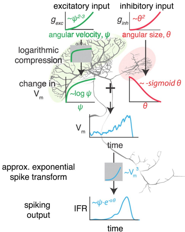
Fig. 1 Computation in the locust's LGMD neurone. When faced with a looming stimulus simulating an object approaching on a collision course, excitatory inputs are received that are proportional to the object's angular velocity raised to a power of 2 or 3. The inhibitory inputs are approximately proportional to the square of the object's angular size. In this biophysical model, the excitatory signal undergoes a logarithmic compression in the excitatory dendritic subfield, while the effect of the inhibitory inputs on the mean resting membrane potential ( V_m ) results in a sigmoidal (nearly linear) dependence on angular size. The sum of these signals in the merge zone (the juncture immediately above the '+' sign) is then exponentiated in the axonal spike initiation zone, resulting in an output relationship that signals an angular threshold size through its firing rate peak ('IFR' stands for instantaneous firing rate). The figure is reprinted from Jones and Gabbiani (2012, Fig. 8) with permission from Gabbiani
